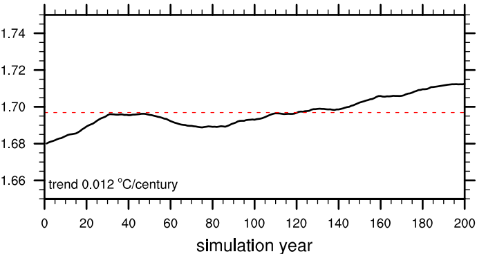
(e) deep ocean temperature averaged below 2500 m
