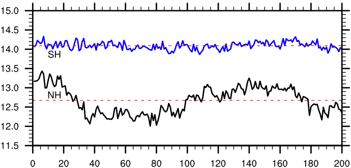
(e) deep ocean temperature averaged below 2500 m
