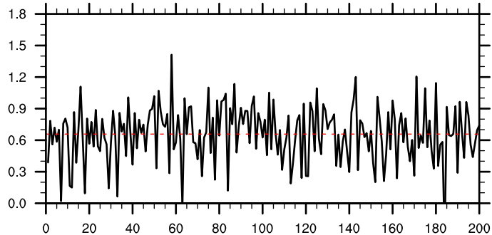
(c) NH and SH surface air temperature
