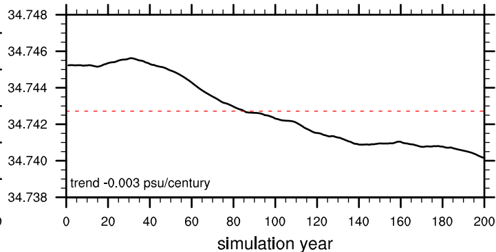
(f) deep ocean salinity averaged below 2500 m
