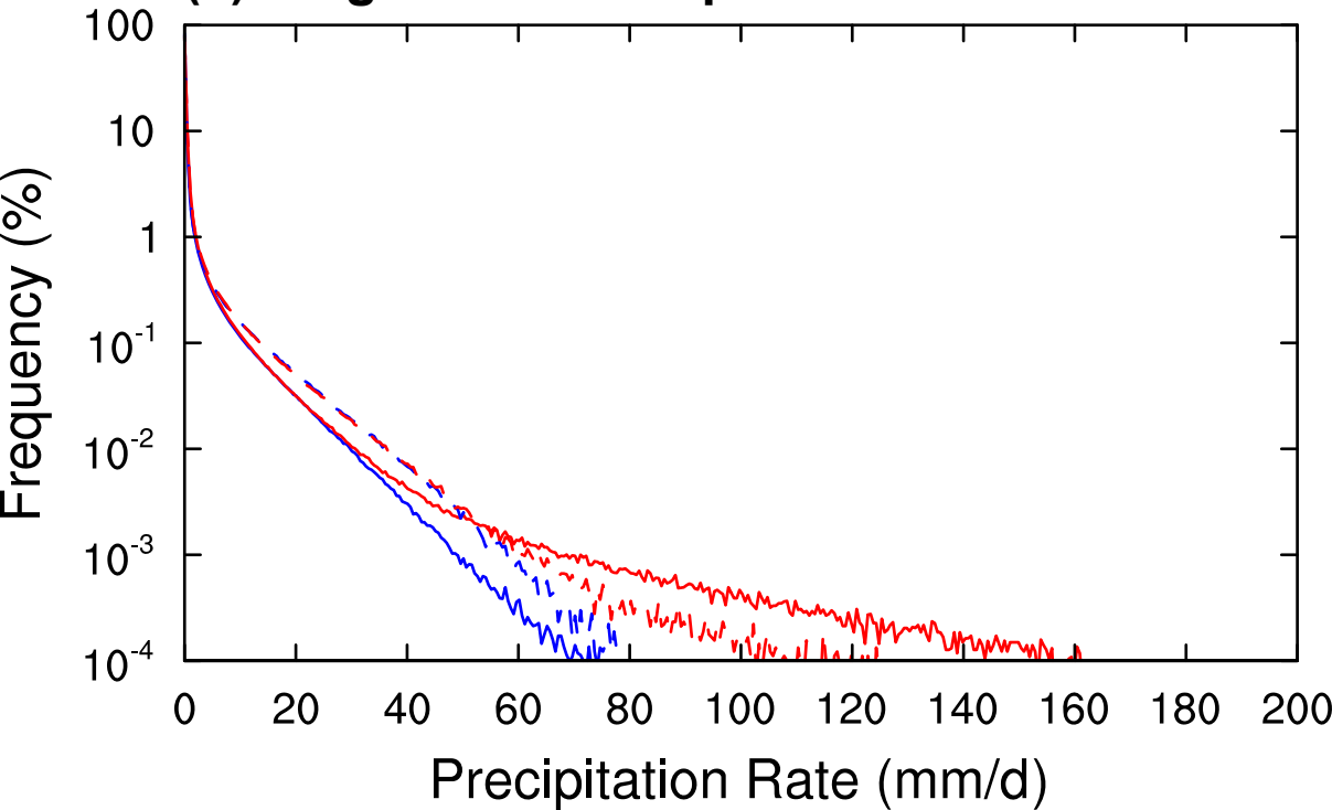
(c) Large-scale Precipitation
