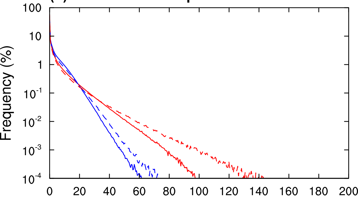
(c) Large-scale Precipitation
