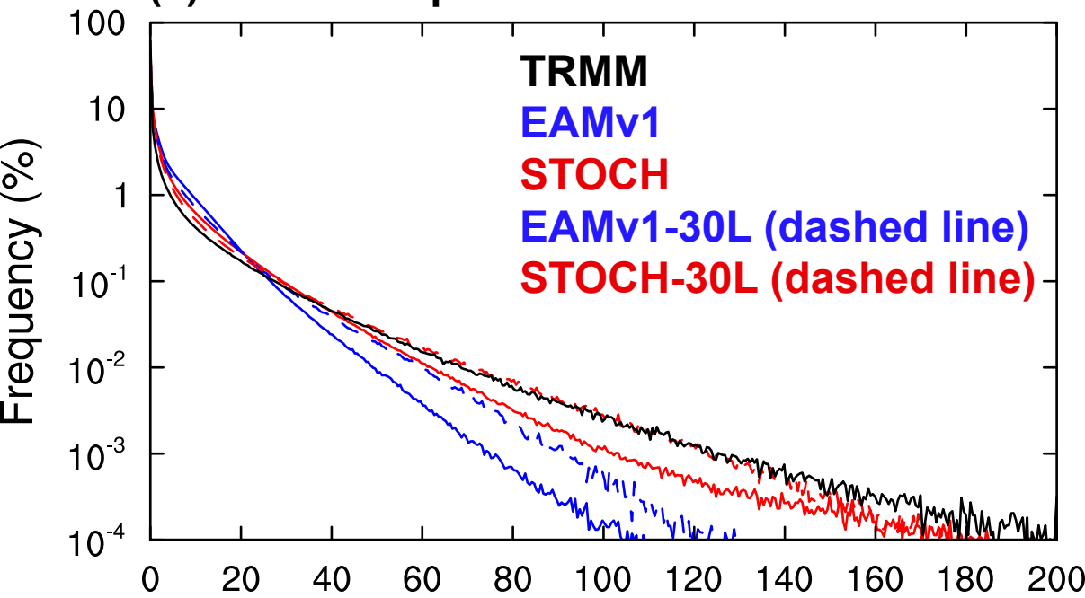
(b) Convective Precipitation
