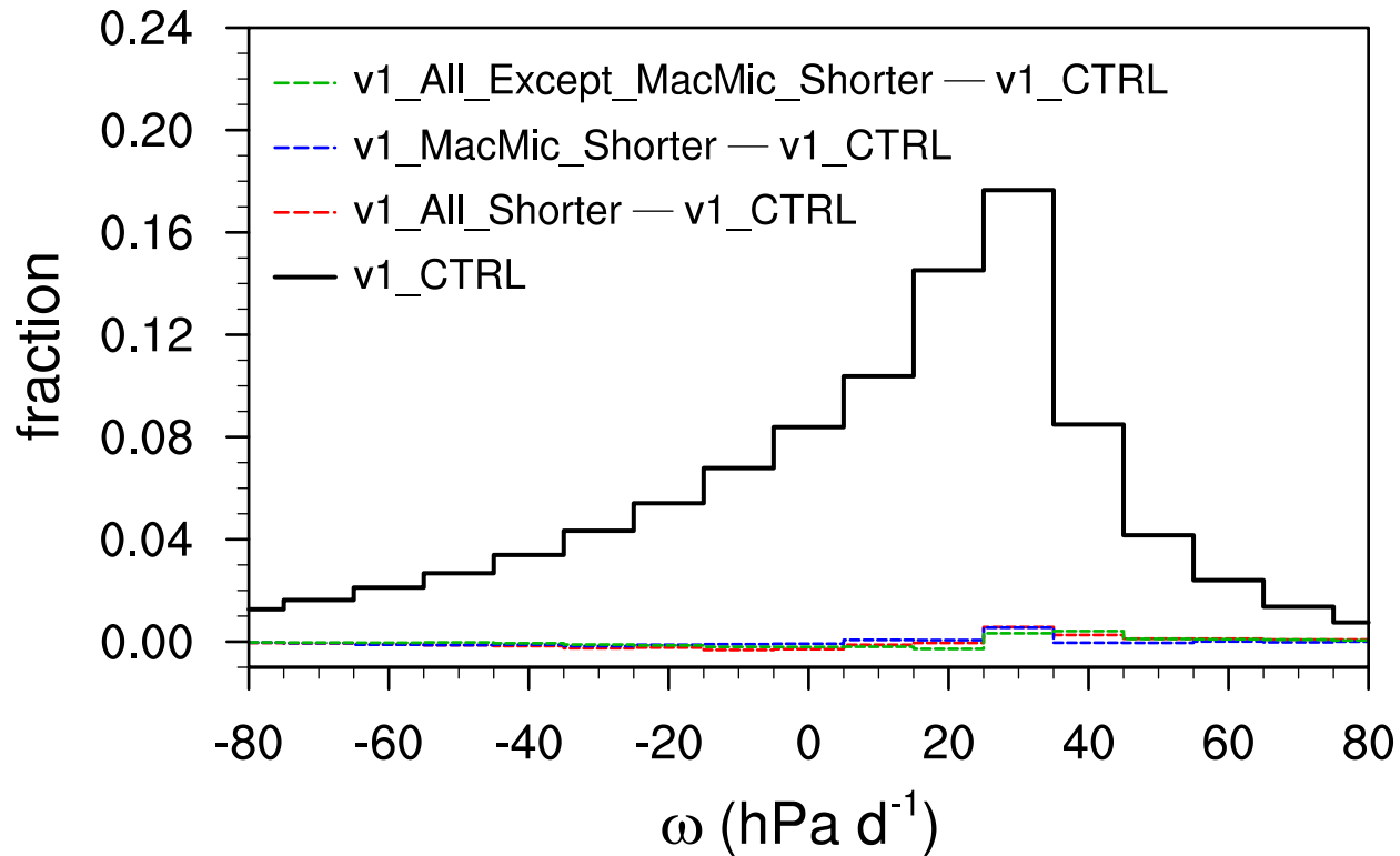
Probability distribution of \omega at 500 hPa
