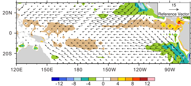
(a) JRA-55
