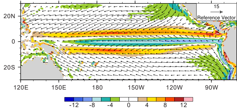
(b) REF_cmp
