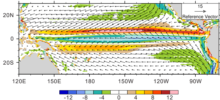
(c) NEW_cmp
