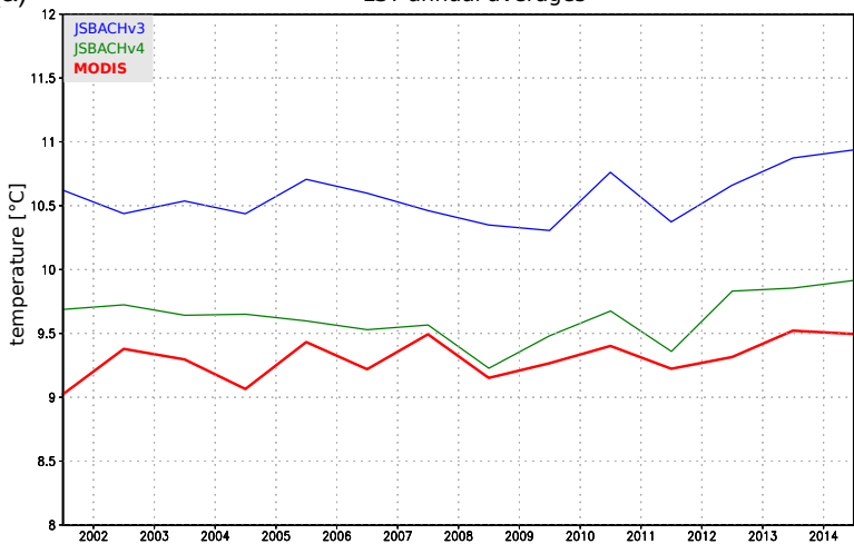
(a) LST annual averages
