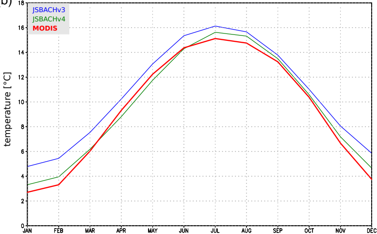
(b) LST seasonal
