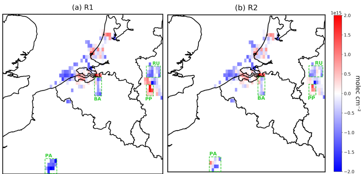
30 Figure S5. Difference between 15-day averaged WRF-Chem and bias-corrected TROPOMI \text{NO}_2 , shown for (a) simulation R1, and (b) simulation R2 using top-down emissions. The dashed green boxes represent four regions of interest: Paris (PA), Brussels-Antwerp (BA), the Ruhr area (RU) and a cluster of power plants in Western Germany (PP). Blank areas are pixels for which the emission adjustment is not considered reliable (see text).
