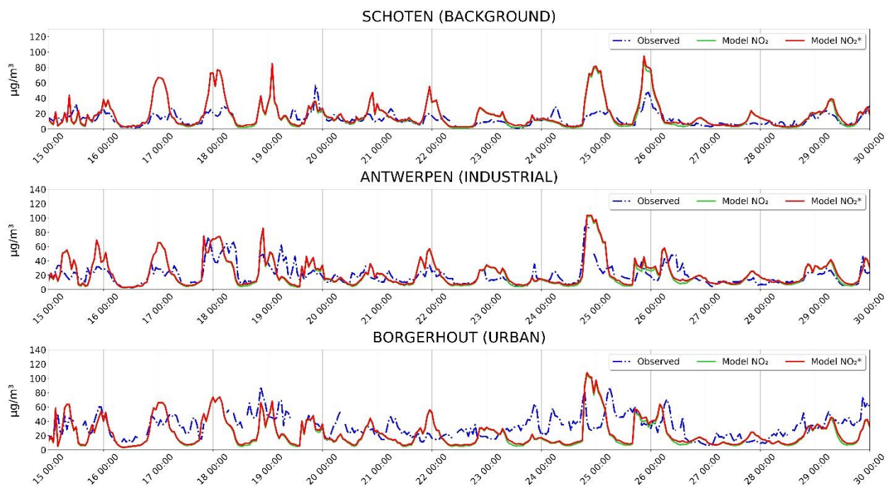
15 Figure S1. Time series of observed and modelled concentrations of NO 2 * at three IRCEL-CELINE network stations: a background site (Schoten), an industrial site (Antwerpen) and an urban one (Borgerhout). Interference-corrected model NO 2 (NO 2 *) is shown in red, and uncorrected NO 2 in green.
