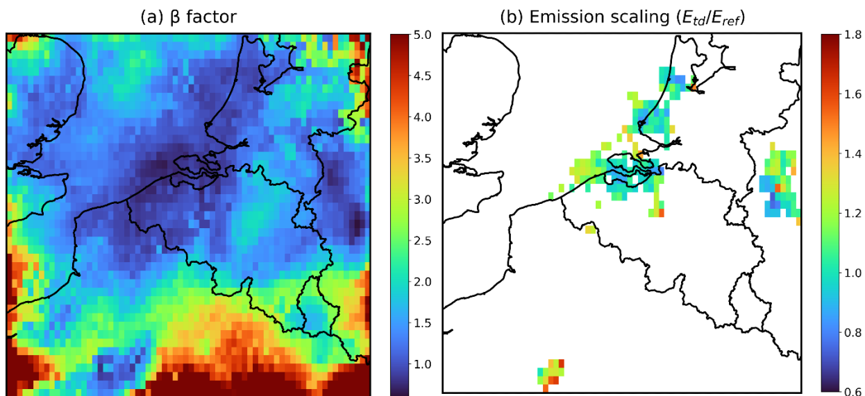
25 Figure S4. Calculated (a) \beta factor and (b) emission scaling factor derived from Eq. 4 in order to improve model agreement with bias-corrected TROPOMI data. White pixels indicate pixels removed due to TROPOMI values being too low ( <4 \times 10^{15} \text{ cm}^{-2} ), or \beta being too high ( >1.45 ). See Section 4.3.3 for details.
