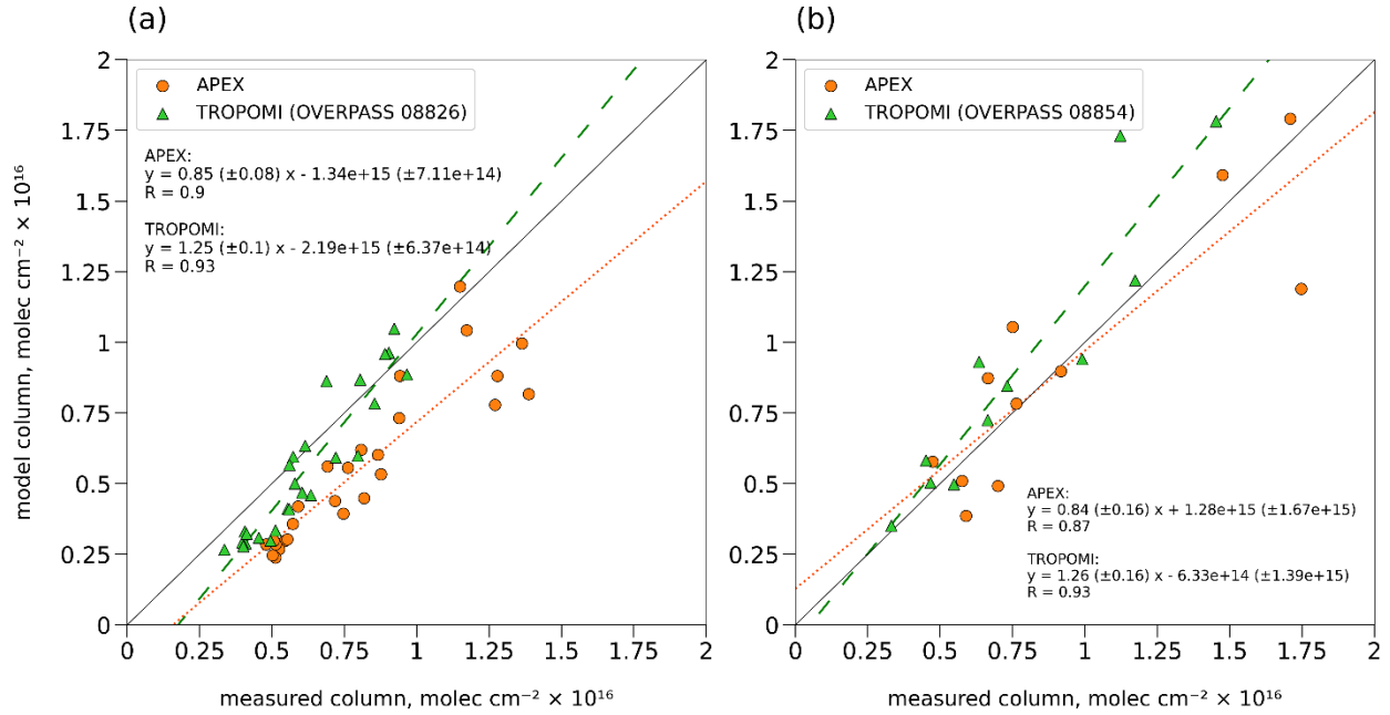
Figure S2. Scatter plots and linear regressions of modelled vs measured columns (APEX and TROPOMI_v1.3) without application of TROPOMI and APEX averaging kernels on model output, on (a) 27th of June and (b) 29th of June. Orange dots and dotted regression lines are for APEX, green triangles and lines for TROPOMI.
