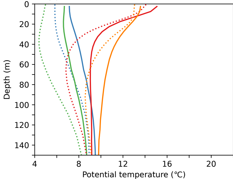
(a) Scotian Shelf--Eastern Gulf of Maine EPU
