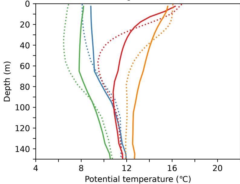
(c) Georges Bank EPU
