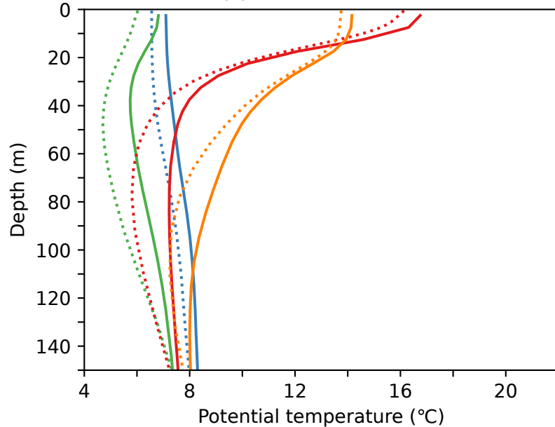
(b) Gulf of Maine EPU
