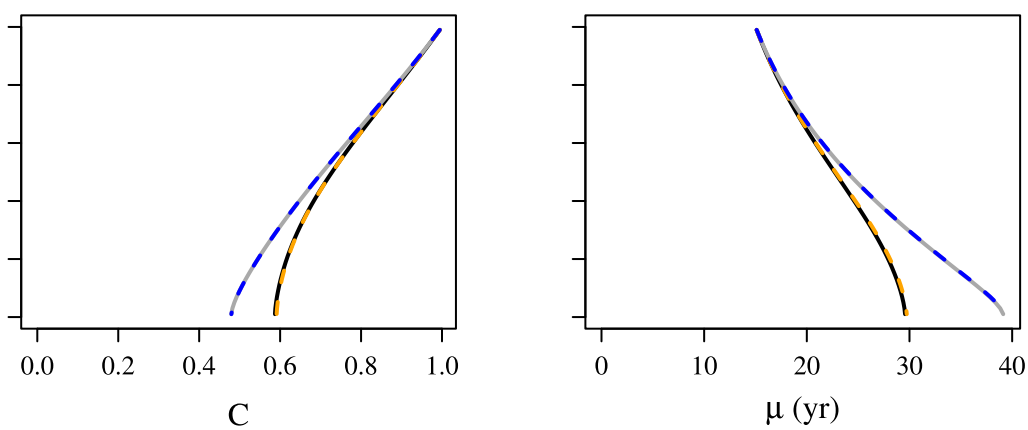
(b) translated Weibull distribution
