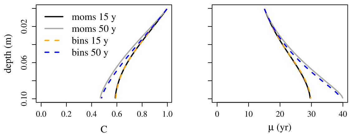
(a) triangular distribution
