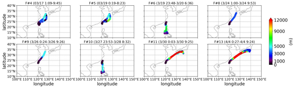
Figure S 6: Crushing altitudes in EMERGE-Asia 2018 campaign.
