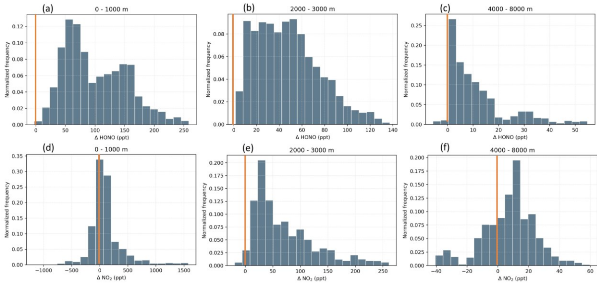
60 Figure S 7: Normalized distributions of the differences between measured and simulated data (OBS - STD) for HONO (upper panel) and NO 2 (lower panel). Data are separated into three categories ( \pm 500 m): 0 - 1000 m (a-d), 2000 - 3000 m (b-e), 4000 - 8000 m (c-f). Three-sigma-rule outlier detection is applied for each altitude range before grouping.
