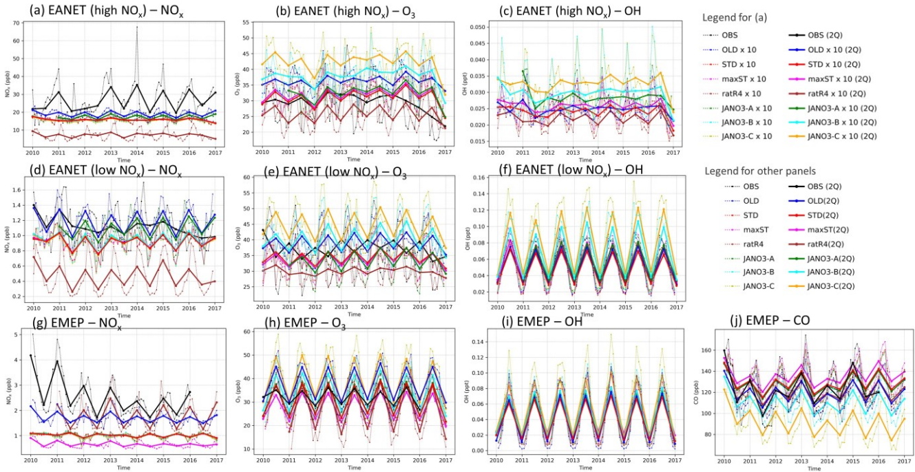
80 Figure S 11: Concentrations of NO x , O 3 , OH, and CO for EANET and EMEP stations by observation and various simulations. The upper legend block indicating simulated NO x concentrations is tenfold for high-NO x EANET stations (a panel). The lower legend block is for the other panels of the figure.
