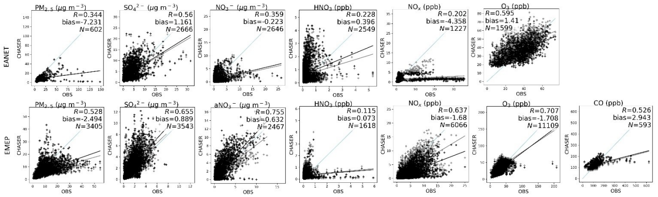
55 Figure S 5: Correlations of STD and OLD runs with EANET (upper) and EMEP (lower) stations for PM 2.5 , SO 4 2- , NO 3 - , HNO 3 , NO x , O 3 , and CO (CO for EMEP only). Fitting lines for STD (black) and OLD (grey) with observations are also plotted. N (no unit) is the number of available data after outlier filtering.
