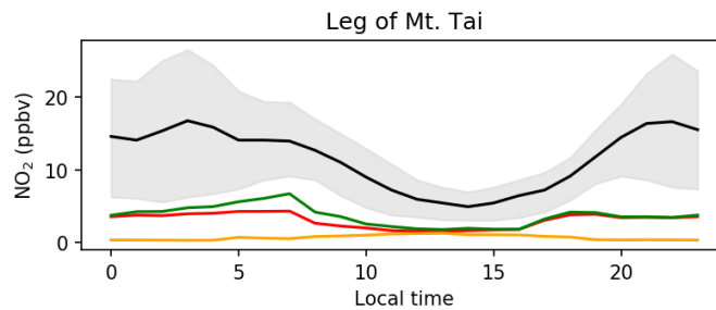
95 Figure S 15: NO 2 concentration at foot of Mt. Tai. At the foot, NO 2 levels in JANO3-A/B/C cases are overlaid by STD case. At the summit, simulated NO 2 levels are nearly zero in all cases (even in the OLD case) while Xue's averaged values were 1.5-3 ppb (minimum and maximum ranged from 0.2 – 5 ppb), thus not be illustrated.
