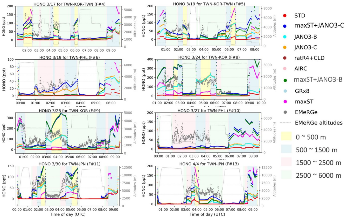
70 Figure S 9: HONO concentrations measured in EMeRGe flights. The observational values (grey dots), the STD case (red), the maxST case (magenta), maxST+JANO3-B case (green lines), and maxST+JANO3-C cases (blue lines) are plotted. Flight altitudes (metres) are plotted in light dash lines scaled to the right axis. Vertical background columns indicate altitude ranges.
