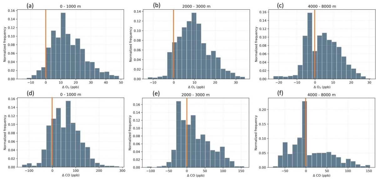
65 Figure S 8: Normalized distributions of the differences between measured and simulated data (OBS – STD) for O 3 (upper panels) and CO (lower panels). Data are separated into three categories ( \pm 500 m): 0 – 1000 m (a-d), 2000 – 3000 m (b-e), 4000 – 8000 m (c-f). Outliers of each altitude group are filtered by a 3-order rule.
