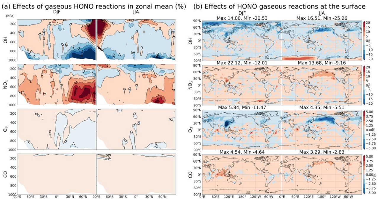
90 Figure S 14: Changes (%) in zonal mean (a) and at the surface (b) for OH, NO x , O 3 , and CO concentrations by gaseous HONO chemistry (R1, R2, R3). The colour scales for each panel are different.
