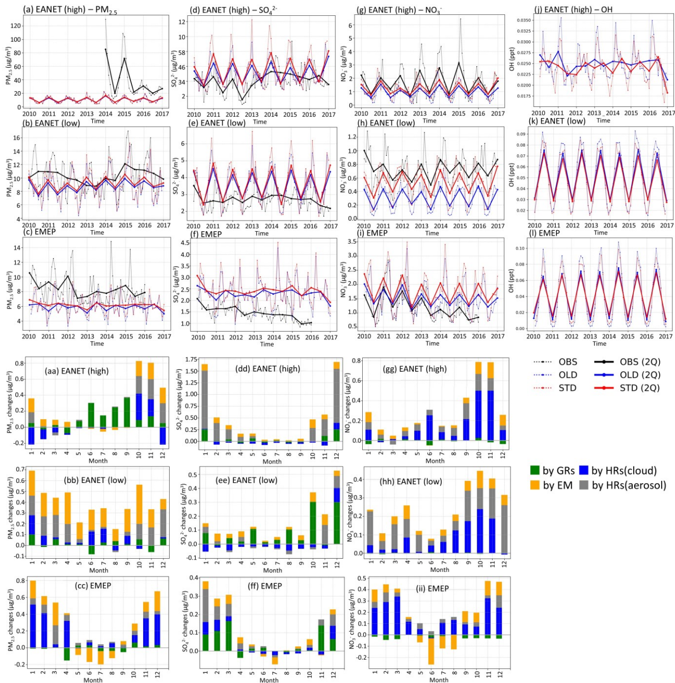
45 Figure S 4: Grouped by observed and simulated mass concentrations (a-l) and monthly-mean changes (aa-ii) for PM 2.5 , SO 4 2- , NO 3 - , and OH for EANET and EMEP stations, grouped as high-NO x EANET, low-NO x EANET, and all EMEP stations. In (a-m), black lines: observation; red: STD case; blue: OLD case. Dotted lines are all stations' median from monthly-mean for each station in that group. Thick solid lines represent two quarters averaged from dotted lines. There are no observational data for OH's plots (j-l), and only values from STD and OLD simulations are presented. In (aa-ii), green bars: monthly changes by GRs; blue: by HRs on clouds; grey: by HRs on aerosols; orange: by EM. 50
