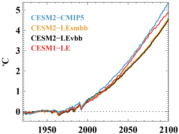
(a) Global \Delta SAT
