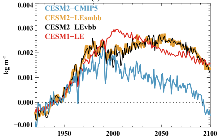
(c) Global \Delta LWP
