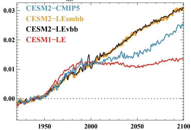
(g) Global \Delta AODVIS
