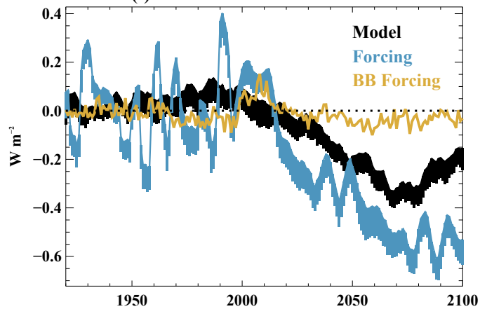
(f) Attribution Global \Delta FSNTC
