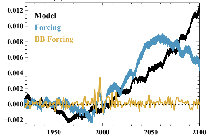
(h) Attribution Global \Delta AODVIS
