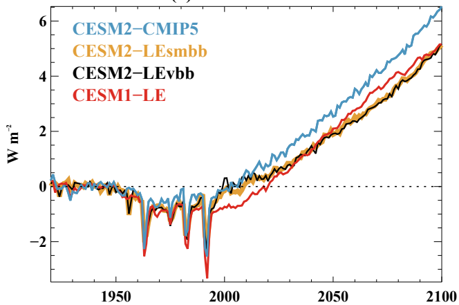
(a) Global \Delta FSNT
