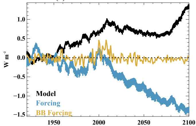
(b) Attribution Global \Delta FSNT
