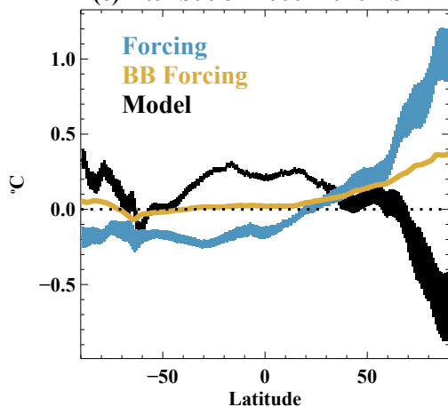
(e) Model Attribution \Delta SAT
