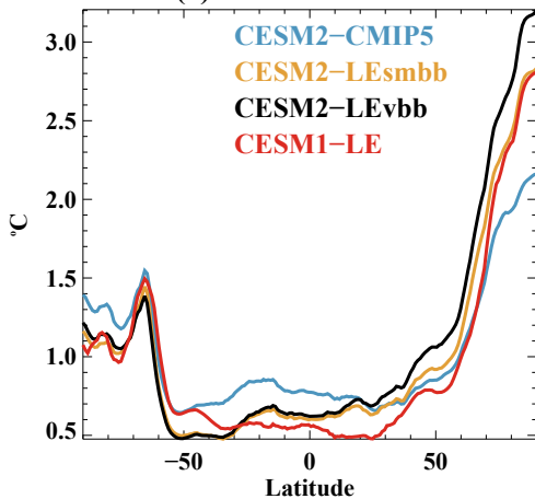
(c) Attribution 2000–2020 \Delta SAT
