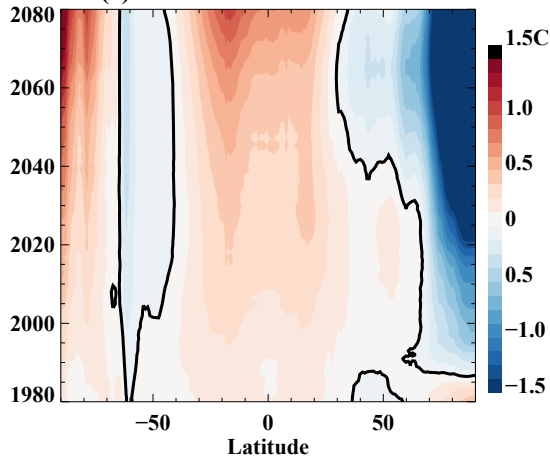
(e) Model Attribution \Delta SAT
