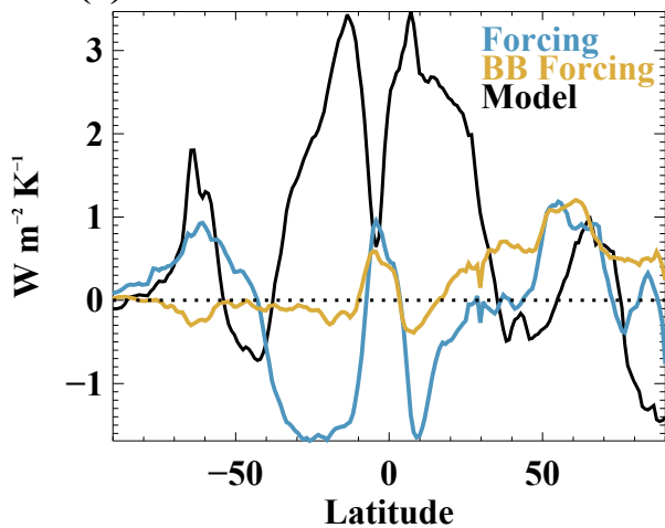
(c) Attribution 2000–2020 CldFB
