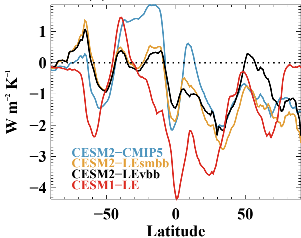
(a) 2000–2020 CldFB
