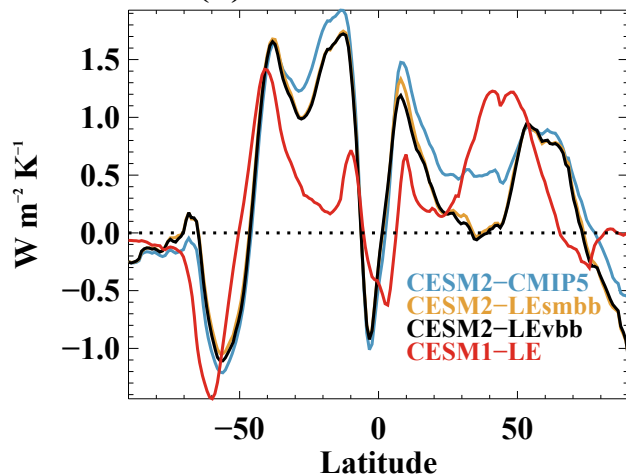
(b) 2080–2100 CldFB
