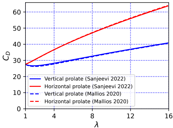
(a) Re = 1
