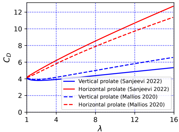
(b) Re = 10
