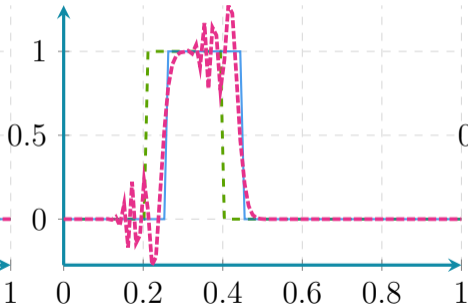
Class 2 - P(X = 2)
