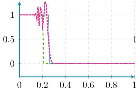
Class 1 - P(X = 1)
