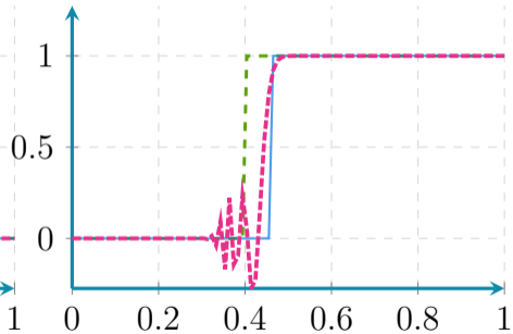
Class 3 - P(X = 3)
