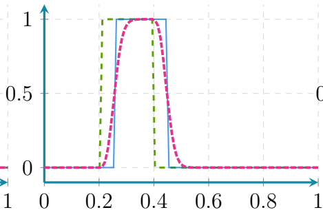
Class 2 - P(X = 2)
