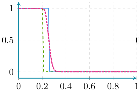
Class 1 - P(X = 1)
