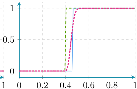
Class 3 - P(X = 3)
