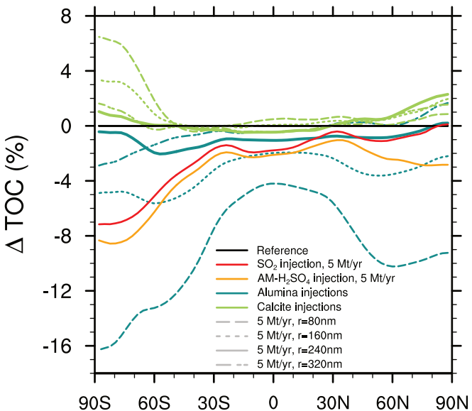
(a) Sensitivity to Particle Radius
