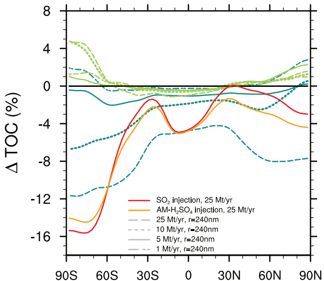
(b) Sensitivity to Injection Rate
