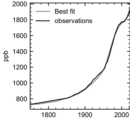
(b) CH 4 concentration
