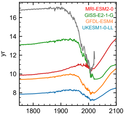
(a) CH 4 lifetime
