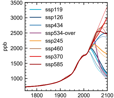
(c) CH 4 projections
