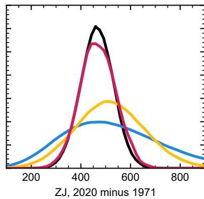
Ocean heat content change
