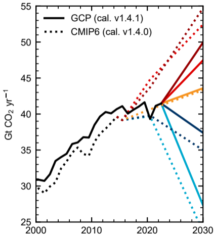
(a) CO 2 emissions
