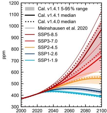
(b) CO 2 concentration
