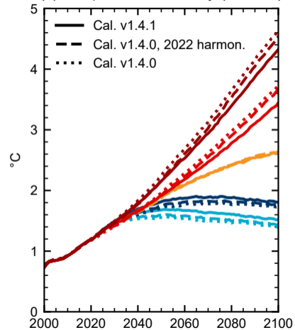
(c) Temperature anomaly (median)
