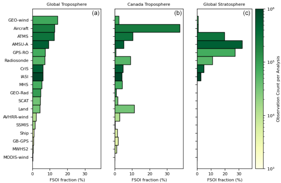
Figure 8. The average fractional observation impact on 24 h forecasts (a) over the global domain and (b) over only Canada between the surface and 100 hPa and (c) for the global domain between 100 and 1 hPa separated by observation type. The colour of each bar indicates the average number of assimilated observations per analysis. The observation types are ordered according to the magnitude of their impact on global tropospheric forecasts.
