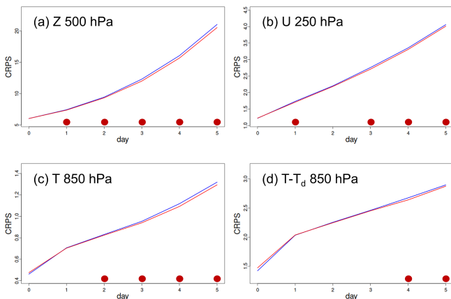
Figure 7. The continuous ranked probability score (CRPS) of 5 d ensemble forecasts from the previous EnKF system (in blue) and the new MIDAS-based LETKF system (in red) computed with respect to the global network of radiosonde observations for (a) geopotential height at 500 hPa, (b) zonal wind at 250 hPa, (c) temperature at 850 hPa, and (d) dew-point depression at 850 hPa over the period 1–25 January 2017. The filled circles along the horizontal axis indicate lead times when the difference in the score is considered statistically significant, with the colour of the circle indicating the experiment with the better score. Note that these results use an earlier configuration of the LETKF and EnKF at lower spatial resolution and without ensemble recentering.
