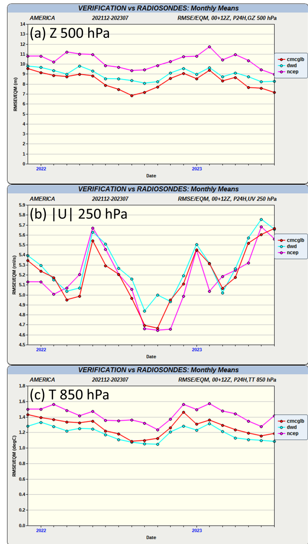
Figure 6. The RMSE of 24 h forecasts from the GDPS (in red) together with the same results from the German Weather Service (in light blue) and the US National Centers for Environmental Prediction (in pink) computed with respect to the North American network of radiosonde observations of (a) geopotential height at 500 hPa, (b) wind speed at 250 hPa, and (c) temperature at 850 hPa. (Note a similar result, but only for 500 hPa geopotential height, is available on the following public website: https://weather.gc.ca/verification/monthly_ts_e.html , last access: 18 December 2024).
