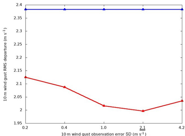
Figure 10. The red line shows the wind gust (10 m a.g.l.) rms departure of the analysis from the withheld observations for different values of the specified observation-error SD when using 10-fold cross-validation over a 2-month period during the winter of 2020. The blue line shows the SD of the observation departure from the HRDPS background state as measured using all of the wind gust observations.
