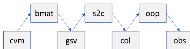
Figure 1. High-level relationship between some of the main MIDAS Fortran modules used for computing an analysis increment or background-error perturbation in observation space (see the main text for definitions of module prefixes). The upper row of modules are transformations between the data-oriented modules in the lower row. Note that each module in the upper row includes “use” statements for the two modules in the lower row to which they are directly connected.
