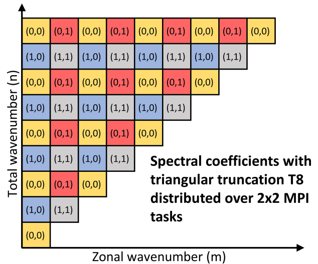
Figure 5. Schematic showing an example of how the spectral coefficients (here up to a triangular truncation of T8, i.e. up to total wavenumber 8) used for the control vector in global variational data assimilation are distributed over the two-dimensional MPI decomposition (here with just 2 \times 2 MPI tasks) following a round-robin strategy. The two values in each box represent the MPI task index over the two dimensions of the decomposition, and a different colour is used to identify each of the four MPI tasks.
