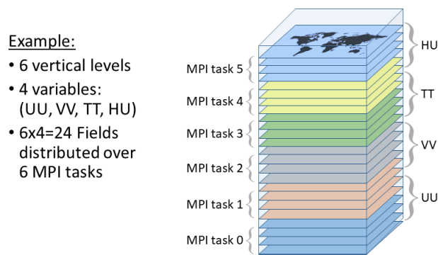
Figure 3. Schematic showing how 2D fields are distributed over MPI tasks with respect to both variables (in this example zonal and meridional wind, temperature, and humidity: UU, VV, TT, and HU, respectively) and vertical levels (six levels in this example). A different colour is used for each MPI task. This data distribution is used when interpolating to observation locations and times.
