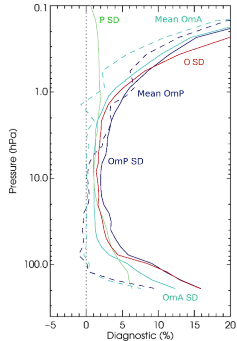
Figure 9. The global normalized mean (dashed) and SD (solid) of MLS observation minus analysis (OmA, light blue) and observation minus short-term forecast (OmP, dark blue) differences and corresponding average observation-error SD (O, red) and background-error SD (P, green) used for assimilation. Results are for the June–August 2022 period.
