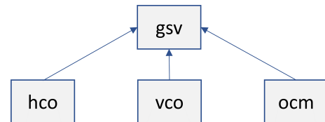
Figure 2. Relationship between the gridded state vector module ( gsv ) and lower-level modules that are used by this module through a composition relationship to represent the horizontal coordinate ( hco ), vertical coordinate ( vco ), and ocean mask ( ocm ).
