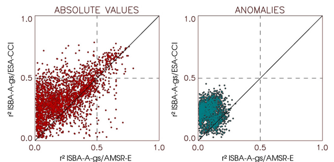
Figure 5. Detrended SSM ESA-CCI vs. AMSR-E, (left panel) absolute and (right panel) anomaly squared correlation coefficients ( r^2 ) with the detrended ISBA-A-gs SSM, over the 2003–2008 period. Note that r^2 values are plotted for grid cells corresponding to positive r values, only.
