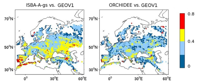
Figure 10. Pearson correlation coefficient ( r ) between the scaled LAI 10-daily anomalies derived from detrended simulations (left, ISBA-A-gs; right, ORCHIDEE) and detrended GEOV1 satellite observations, over the 1991–2008 period, at grid cells presenting significant positive correlations ( p value < 0.01 ).
