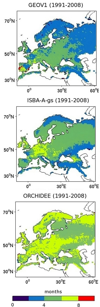
Figure 7. Same as Fig. 6, except for LGP values.
