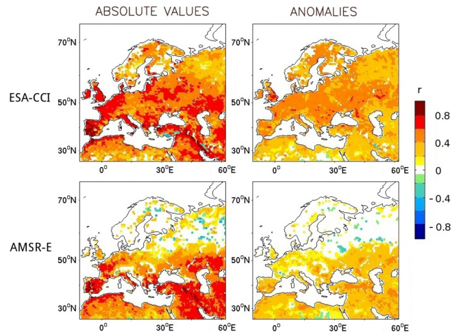
Figure 4. Same as Fig. 3, except for the 2003–2008 period and (top) ESA-CCI vs. ISBA-A-gs, (bottom) AMSR-E vs. ISBA-A-gs.
