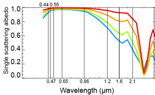
Figure 9. OPAC single scattering albedo as a function of humidity (color) and wavelength. The various relative humidity levels are in order (red, orange, green, and blue) for 95, 80, 30, and 0% column relative humidity.
