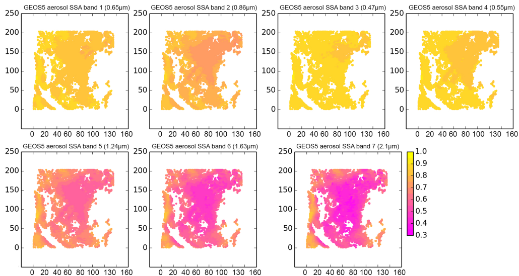
Figure 7. Bulk aerosol single scattering albedo for Brazil 1 case for MODIS channels 1–7. This single scattering albedo combines all aerosol species present in the scene.
