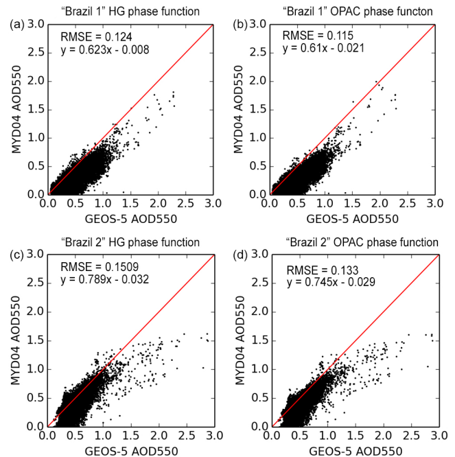
Figure 5. Effect of aerosol phase function shape on Brazil smoke cases. Panels (a) and (c) show the runs with HG phase function. Panels (b) and (d) show use of the OPAC composite phase function.
