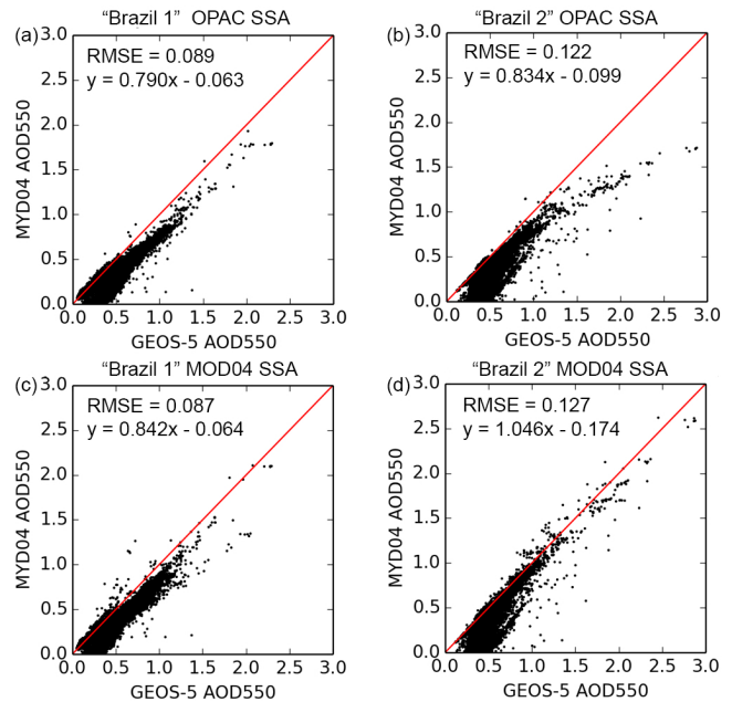
Figure 10. Impact of humidity on MOD04 retrieval illustrated via single scattering albedo selection. Panels (a) and (c) show the Brazil 1 case before and after the SSA adjustment. Panels (b) and (d) show the same for Brazil 2.
