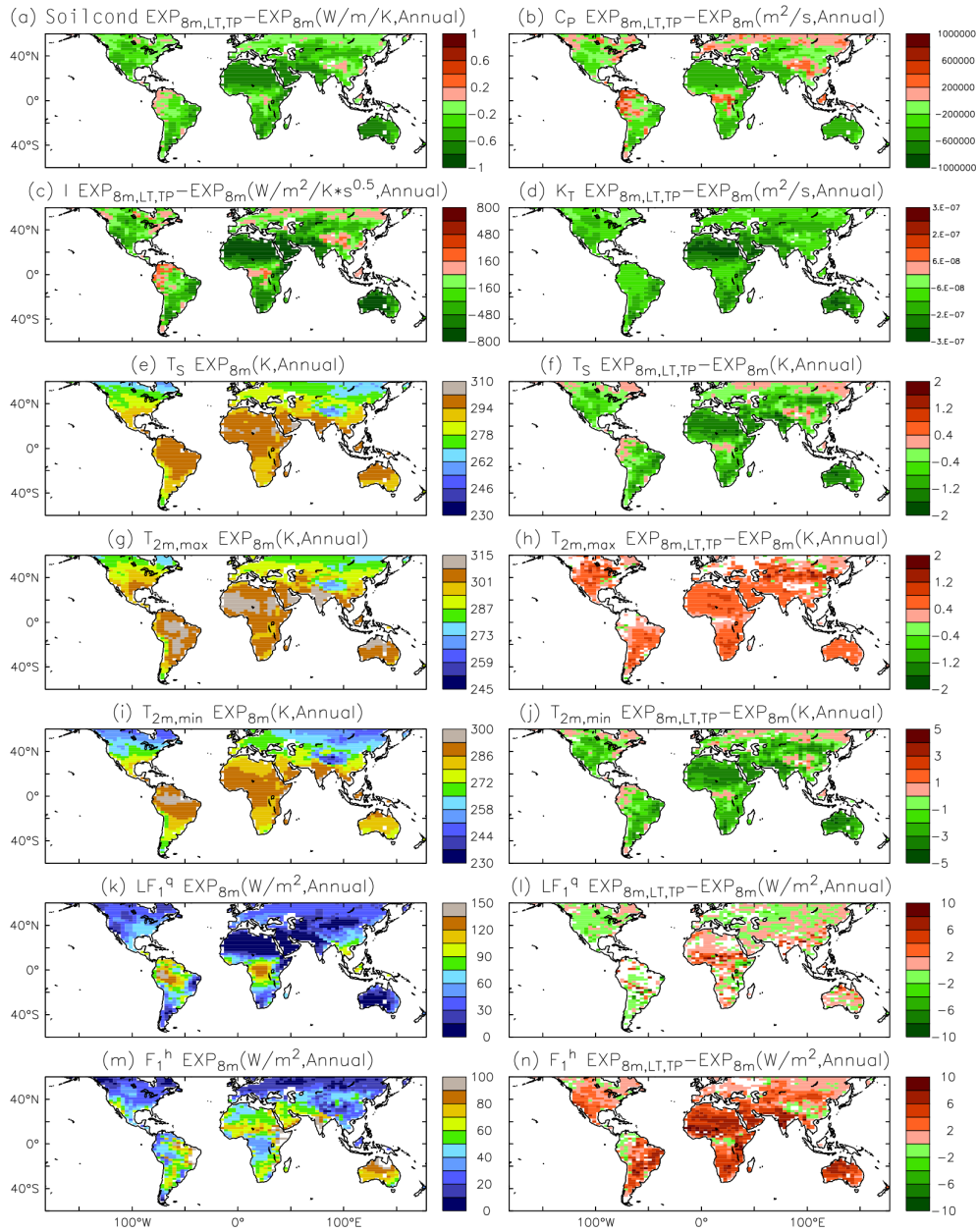
Figure 8. The LMDZOR simulations (annual mean) for EXP 8m (left) and the differences between EXP 8m,LT,TP (Table 4) and EXP 8m (right) for (a) soil thermal conductivity, (b) soil heat capacity, (c) soil thermal inertia, (d) soil heat diffusivity, (e, f) surface temperature, (g, h) daily maximum temperature, (i, j) daily minimum temperature, (k, l) latent heat flux, and (m, n) sensible heat flux. The white regions indicate that the new parameterizations are not significant.
