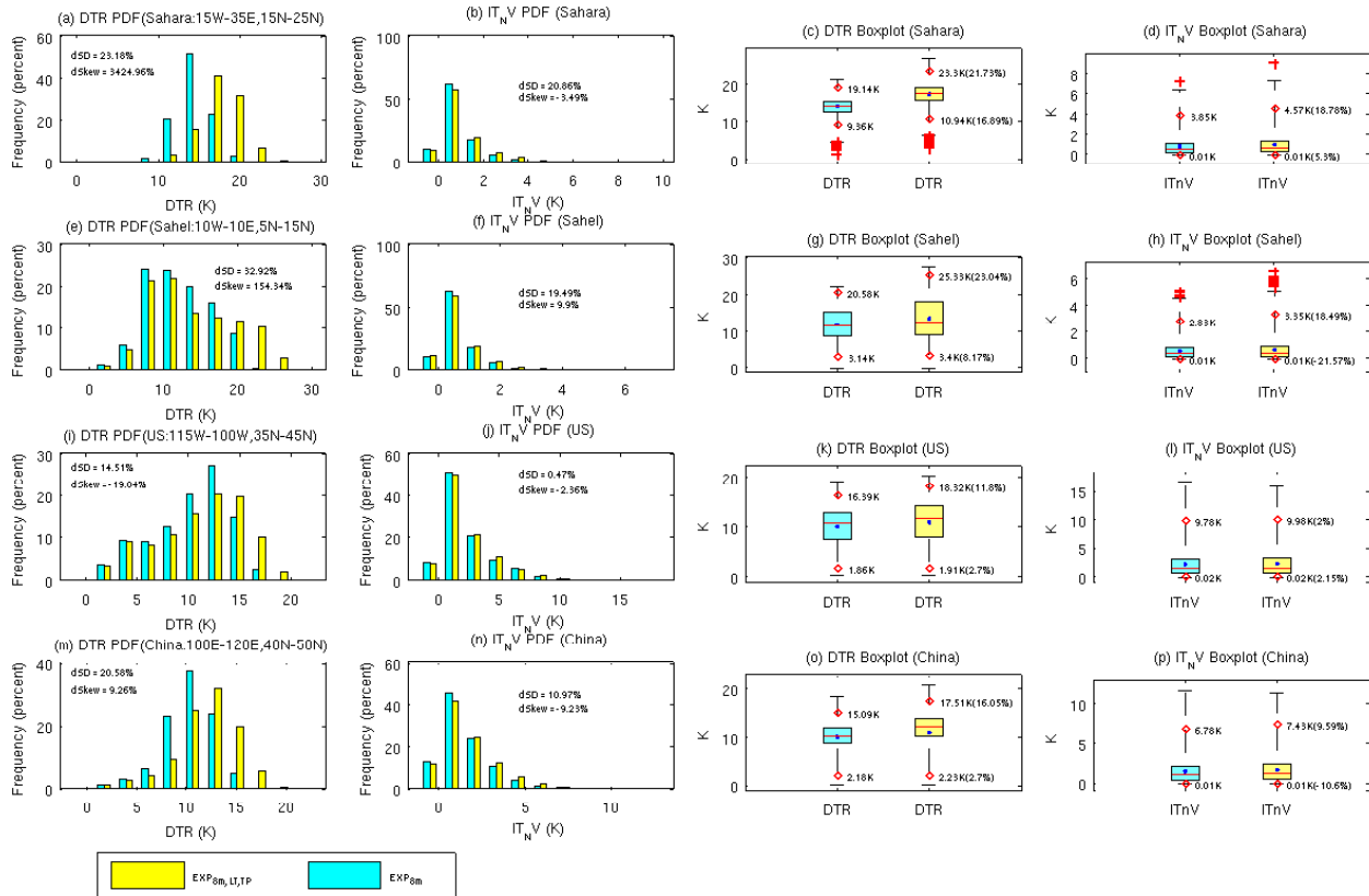
Figure 10. The probability density function (PDF) for DTR (1 column) and IT_{N,V} (2 column), and the box plot of DTR (3 column) and IT_{N,V} (4 column) over the Sahara (1 line), the Sahel (2 line), the central US (3 line), and North China (4 line) between EXP_{8m,LT,TP} (in yellow) and EXP_{8m} (in blue) with daily values. The grid point value is weighted by its areas. In the box plot, the red central mark and the blue dot are the median and mean, and the edges of the box and the 25 and 75 percentiles. The whiskers extend to the most extreme data points not considered outliers. Points are drawn as outliers if they are larger than X_{75th} + 3 \cdot (X_{75th} - X_{25th}) or smaller than X_{25th} - 3 \cdot (X_{75th} - X_{25th}) , where X_{25th} and X_{75th} are the 25 and 75 percentiles, respectively. The red diamond and the values are the 99 and 1 percentiles. The percentage (%), dSD, dSkewness in PDF; values in brackets in box plot) measures the difference between the two simulations: (EXP_{8m,LT,TP} - EXP_{8m})/EXP_{8m} \cdot 100\% .
