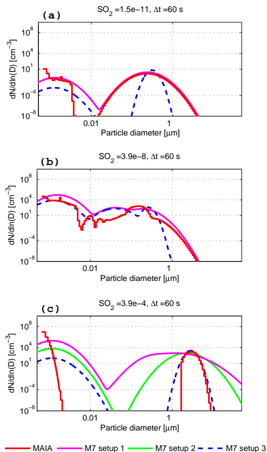
Fig. 3. The aerosol number size distribution at noon of the 10th day of the simulation calculated using the reference model MAIA and M7 with three different different mode setups for different initial \text{SO}_2 concentrations: (a) 1.5 \times 10^{-11} kg/kg, (b) 3.9 \times 10^{-8} kg/kg, and (c) 3.9 \times 10^{-4} kg/kg.
