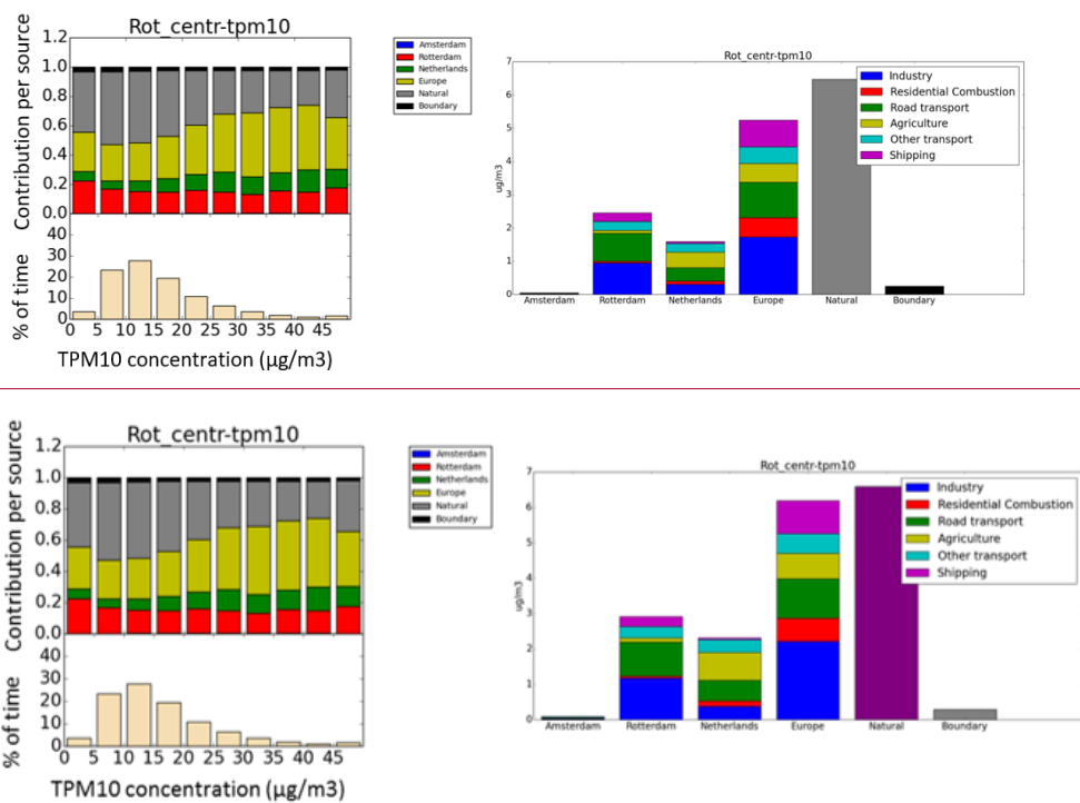
Figure 7. Source apportionment for Rotterdam City Centre, 2011. Relative contribution of several source sectors to daily average PM 10 concentrations (left) and annual average absolute contributions of PM 10 from several source regions and sectors (right). Note that the natural and boundary contributions have by construction no contributions of sectors or countries.
