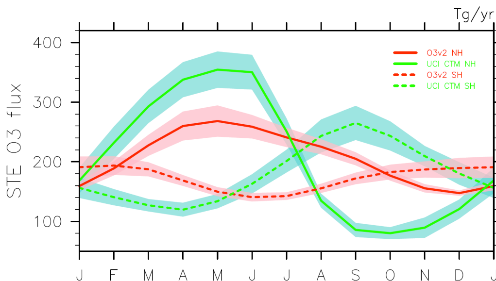
10 Figure 6: Mean annual cycle of the stratosphere troposphere exchange (STE) ozone fluxes (unit: Tg O 3 /yr) at NH (solid lines) and SH (dashed lines) for O3v2 (red) and UCI CTM (green). The lines indicate the climatology mean, and shaded area covers the mean \pm 1 STD.
