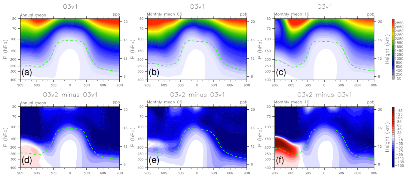
Figure 7: Zonal mean SCO profiles from O3v1 (top) and O3v2 minus O3v1 (bottom) at the upper troposphere/lower stratosphere (UT/LS) region for annual, June, and October means.
