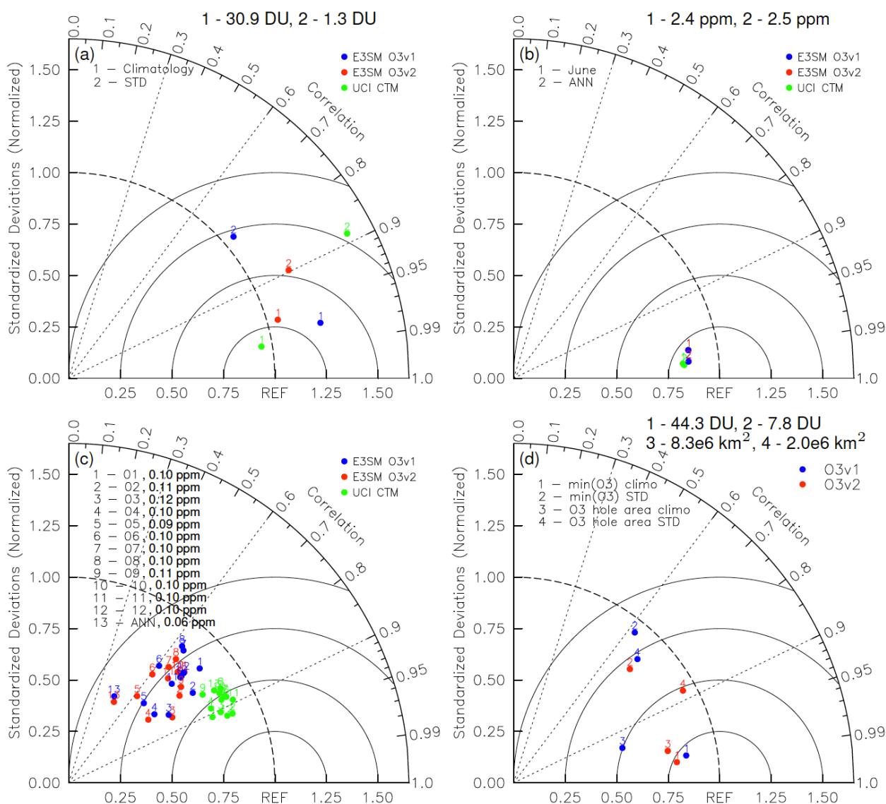
5 Figure 3: Taylor diagrams of (a) area-weighted multi-year annual cycle of SCO (Figure 1) and area-weighted year-to-year standard deviation of the SCO monthly anomalies (Figure 2) with the OMI+MLS observations as the reference point (1,0); (b) area-weighted multi-year zonal mean stratospheric ozone abundances (Figure 4) relative to the MLS observations. Results are shown only for annual and June means, other months are similar; (c) area-weighted year-to-year standard deviation of the zonal mean stratospheric ozone abundances relative to the MLS observations; (d) daily Antarctic ozone hole diagnostics (Figure 5) relative to the NASA ozone watch data. Numbers 1 and 3 are for the daily mean time series, while numbers 2 and 4 represent the daily STD time series. On all Taylor diagrams, the model STDs are normalized by dividing the STDs of the reference (labeled with units).
