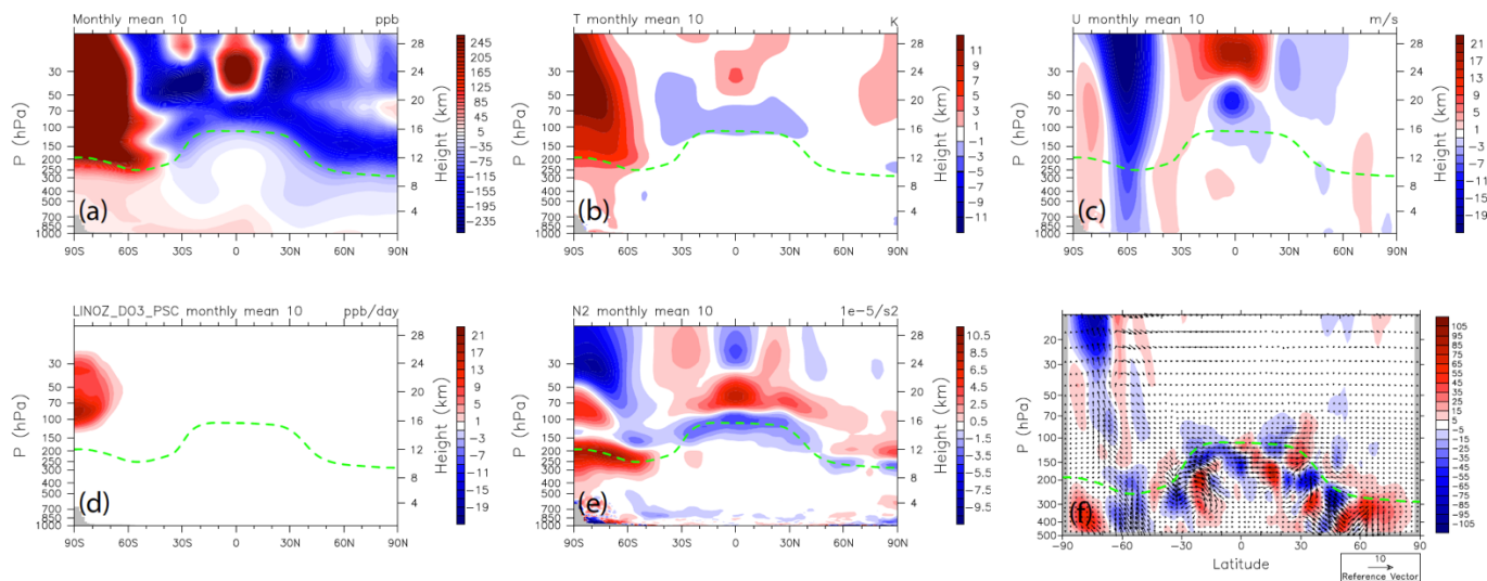
Figure A1: Pressure by latitude mean differences between O3v2 without retuning the PSC T threshold and O3v1 in October of 5 weak ozone hole years (1998, 2001, 2007, 2011, 2013) for (a) O 3 , (b) temperature, (c) zonal wind, (d) PSC ozone loss tendency, (e) buoyancy frequency squared (N 2 ), and (f) E-P flux vector and divergence.
