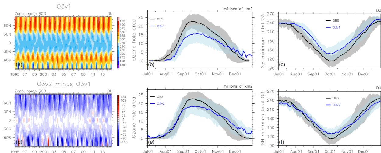
5 Figure 5: (left) Time series of zonal mean SCO by latitude (unit: DU) showing Antarctic ozone hole over years 1995–2014 and (middle) daily evolution of the ozone hole from July 1 to December 31 as measure by area ( 10^6 km 2 ), and (right) minimum total column ozone (DU). Results are shown for models E3SM O3v1 (top row) and O3v2 (bottom row). Results for UCI CTM are not shown because daily diagnostics were not saved. Observations from the NASA ozone watch data for 1990–2019 are also shown in the right two columns. The lines indicate the multi-year mean (observations in black; models in blue), and shaded area covers \pm 1 standard deviation.
