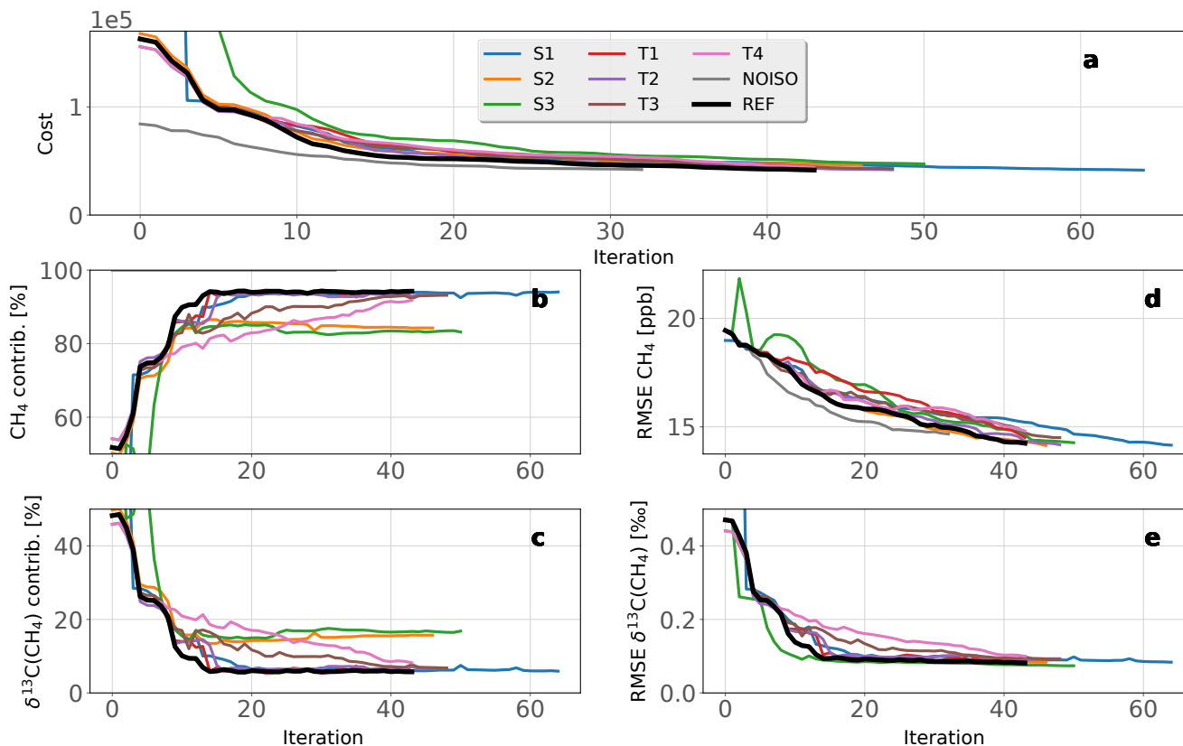
Figure 3. Minimization of the cost function for all configurations. a) Value of the cost function with respect to the number of iterations. b) \text{CH}_4 contribution to J_o . c) \delta^{13}\text{C}(\text{CH}_4) contribution to J_o . d) RMSE associated to observed-simulated \text{CH}_4 . e) RMSE associated to observed-simulated \delta^{13}\text{C}(\text{CH}_4) . For clarity reasons, S1 and S3 initial values are not displayed because they are much larger than those of REF.
