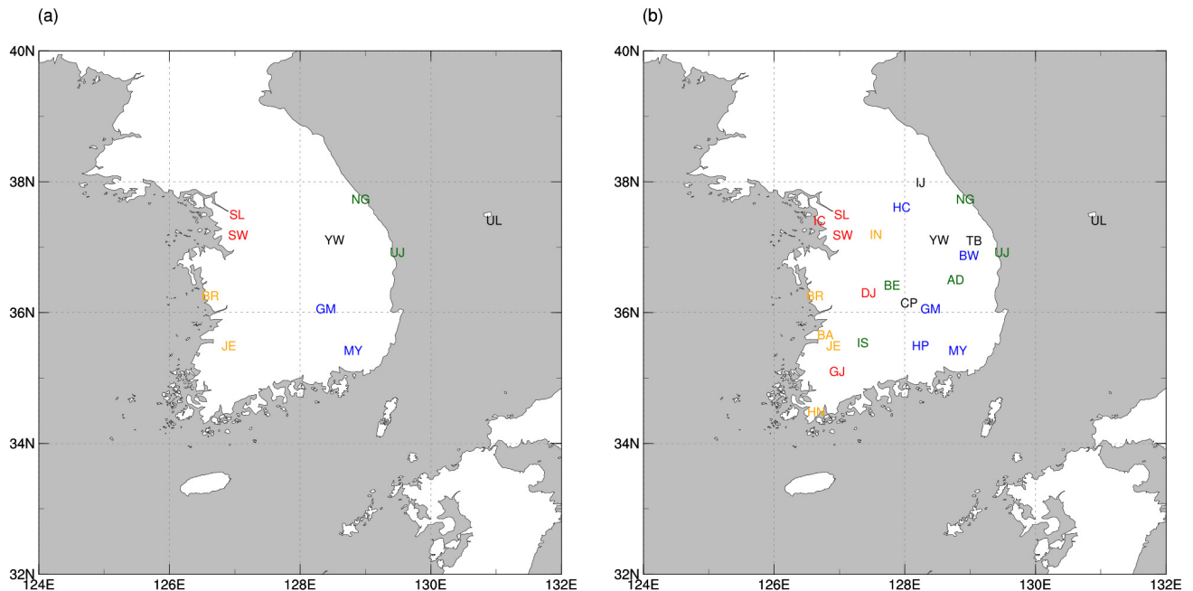
Figure 3. Stations used for the experiments (a) CNTL-OPT_5 and (b) OPT_6W, CNTL_VRF_5 and (b) OPT_VRF_W6. Different colors in the station acronyms represent different land-cover types (LCT): DBF (black), MF (blue), WS (dark-green), CL (yellow), and UB (red). See Table 1 for the acronyms of stations and land-cover types (LCTs).
