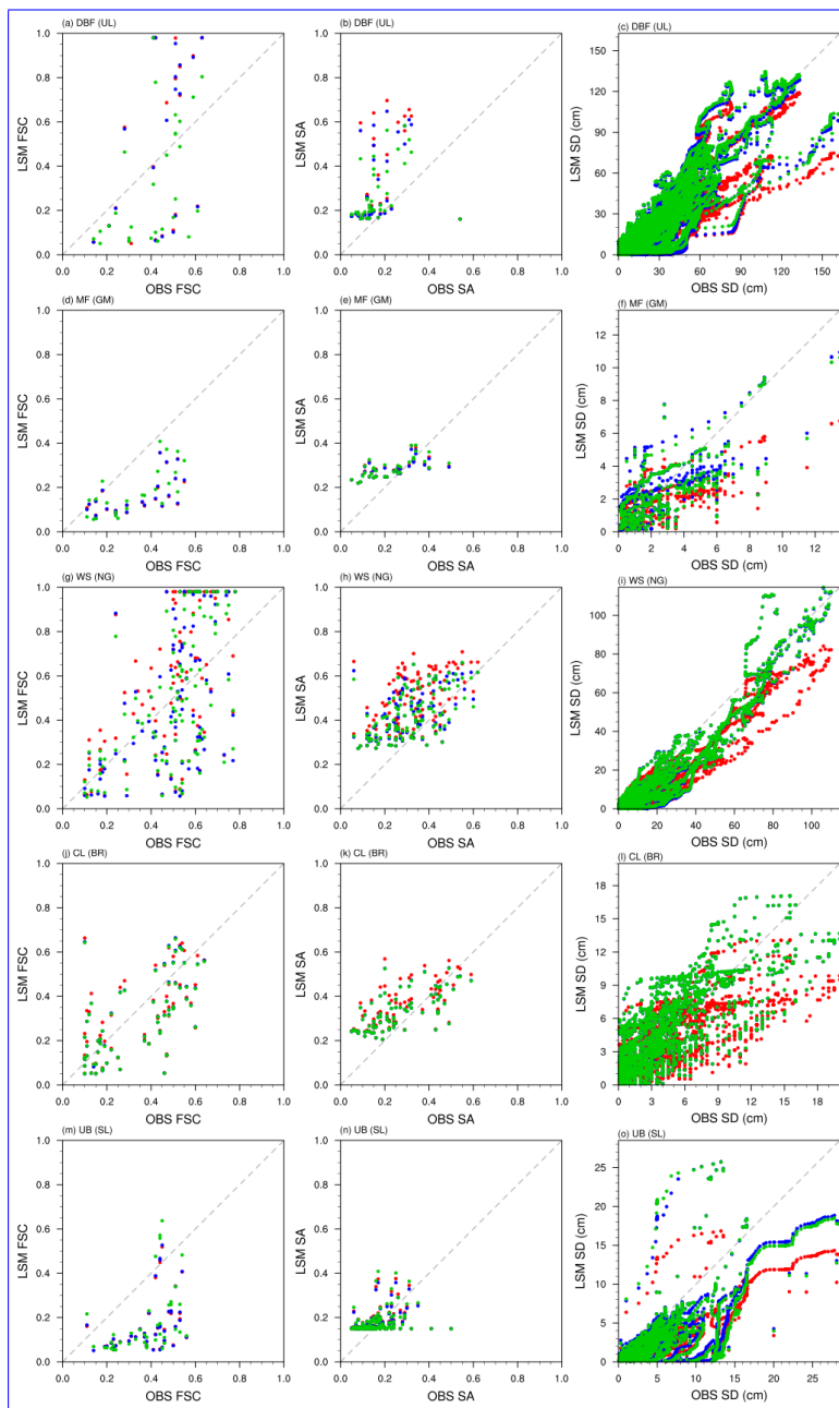
Figure 6. Scatter plots for the observation of observations (OBS) and land surface-model results (LSM) results for snow variables FSC (left panels), SA (middle panels), and SD (in cm; right panels) from the verification experiments — CNTL (red dots), OPTVRF_5 (blue dots), and OPTVRF_6 (green dots). The representative station in each land cover type, which are analyzed such as evaluated over different LCTs; (aa-c) - (e) DBF represented by the station UL, (dd-f) - (f) MF by GM, (gg-i) - (i) WS by NG, (jj-l) - (l) CL by BR, and (mm-o) - (o) UB by SL. From the left to right panels, they are the
