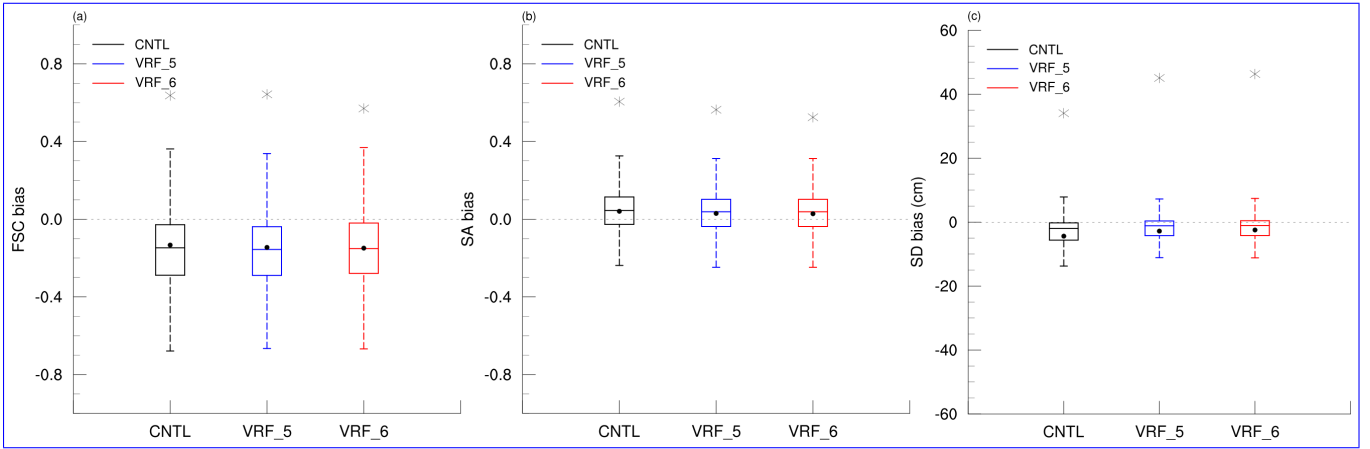
Figure 5. Box plots of (a) FSC bias, (b) SA bias, and (c) SD bias (cm) for CNTL, \text{OPTVRF}_5 and \text{OPTVRF}_6 . The maximum differences are indicated with the black star symbol (e.g., 0.637 (CNTL), 0.643 ( \text{OPTVRF}_5 ), 0.570 ( \text{OPTVRF}_6 ) for FSC, 0.605 (CNTL), 0.563 ( \text{OPTVRF}_5 ), and 0.525 ( \text{OPTVRF}_6 ) for SA, and 34.1 cm (CNTL), 45.1 cm ( \text{OPTVRF}_5 ), and 46.3 cm ( \text{OPTVRF}_6 ) for SD). Each mean of snow variables is indicated as a black circle (e.g., -0.107 – -0.133 (CNTL), -0.125 – -0.145 (OPT_5), and -0.130 – -0.149 ( \text{OPTVRF}_6 ) for FSC, 0.0513 – 0.0408 (CNTL), 0.0381 – 0.0298 ( \text{OPTVRF}_5 ), and 0.0359 – 0.0281 ( \text{OPTVRF}_6 ) for SA, and -5.38 – -4.39 cm (CNTL), -3.46 – -2.81 cm ( \text{OPTVRF}_5 ), and -2.93 – -2.45 cm ( \text{OPTVRF}_6 ) for SD).
