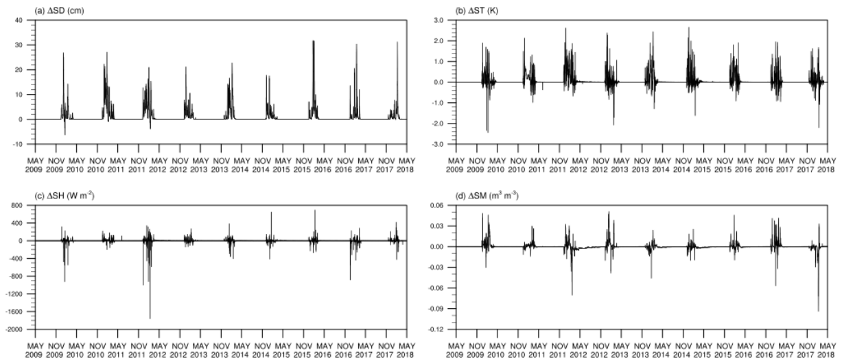
Figure 8. Time series of difference between CNTL to OPTVRF 6 for the UL in DBF during the May 2009 to April 2018: (a) SD (cm), (b) soil temperature at the top soil layer (7 cm) (ST; K), (c) Sensible sensible heat flux (SH; \text{W m}^{-2} ), (d) soil moisture at the top soil layer (7 cm) (SM; \text{m}^3 \text{m}^{-3} ).
