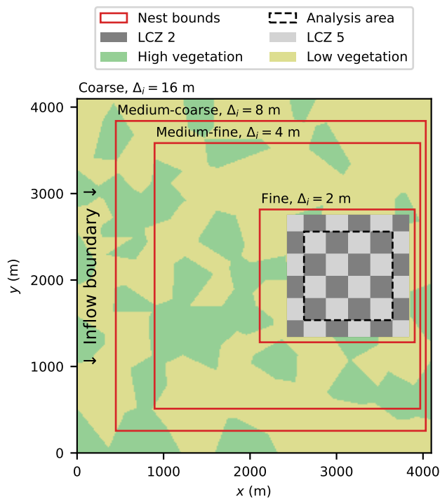
Figure 5. A schematic overview of the modelling approach for the model comparison, representing a mosaic of urban patches surrounded by mixed vegetation patches. The vegetation cover is simplified into two categories for the purpose of clarity, while the vegetation cover used in the simulations follows that used in the precursor (see Appendix B for further details).
