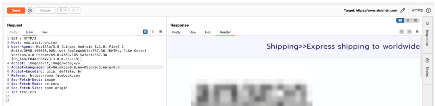
Figure 7: The scam websites still presented their fake e-commerce pages when accessed via desktop browser and Facebook ad lure — provided the browser's user agent (line 3, upper left) was configured to imitate a mobile device (Source: aisicheh[.]com )
