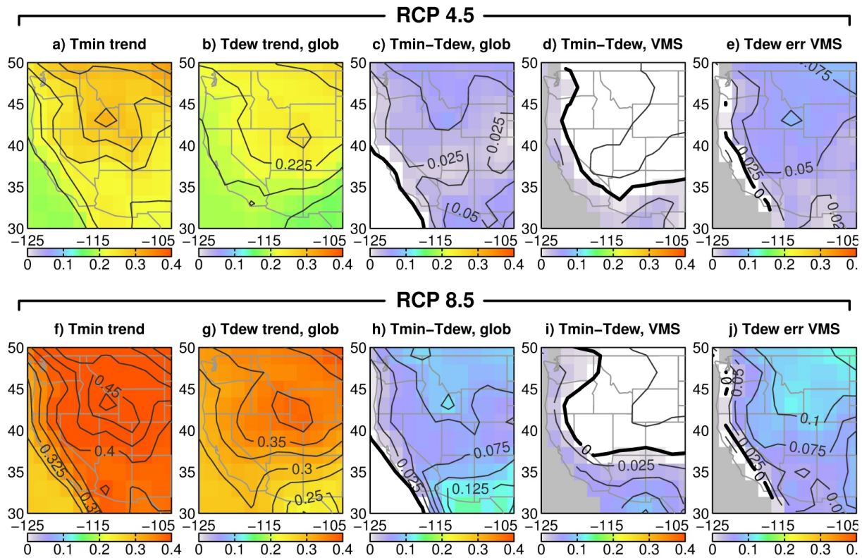
Fig. 11. For the mean of the global models, using RCP 4.5 forcing: (a) the T_{\min} trend, °C per decade; (b) T_{\text{dew}} trend from the global model, °C per decade; (c) T_{\min} trend minus global model T_{\text{dew}} trend, °C per decade; (d) T_{\min} trend minus VMS's T_{\text{dew}} trend, °C per decade. (e) Error in VMS's T_{\text{dew}} trend (with respect to the global model), °C per decade. Panels (f)–(j): same, but for RCP 8.5 forcing. Contour interval is 0.025.
