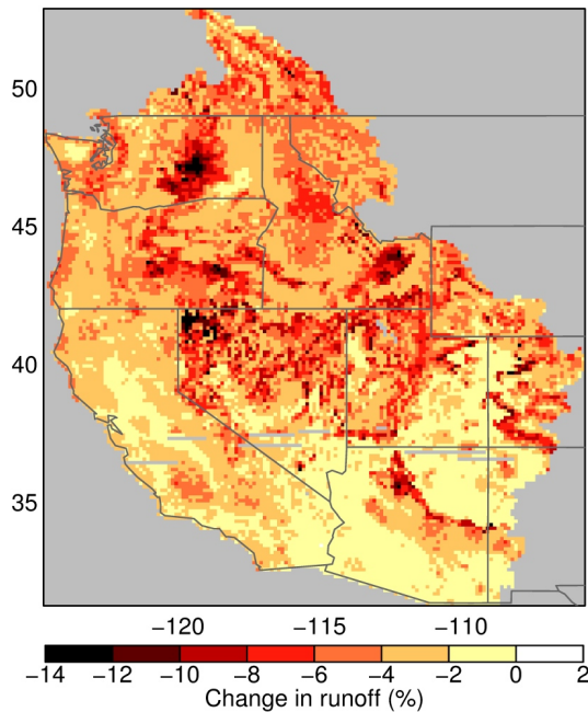
Fig. 13. Changes in annual runoff (%) calculated by VMS given an imposed, fixed 0.75\text{ °C} decrease in T_{\text{dew}} .
