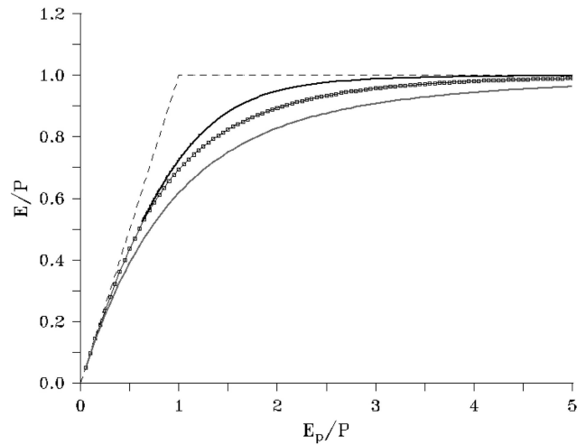
Figure 3. Prototype Budyko curves for the baseline prototype, i.e., \eta = 4 , in the formulation of runoff (thick black), for Eq. (15) for \eta = 2 (gray), and Budyko’s empirical formula (squares). The dashed lines are the energy- and water-limited asymptotes.
