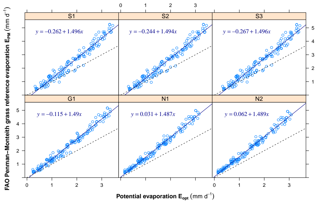
Figure S2: Comparison of potential evaporation estimates for vegetation period in 2013 for each site. The FAO Penman-Monteith grass reference evaporation is plotted as a function of E_{opt} .
