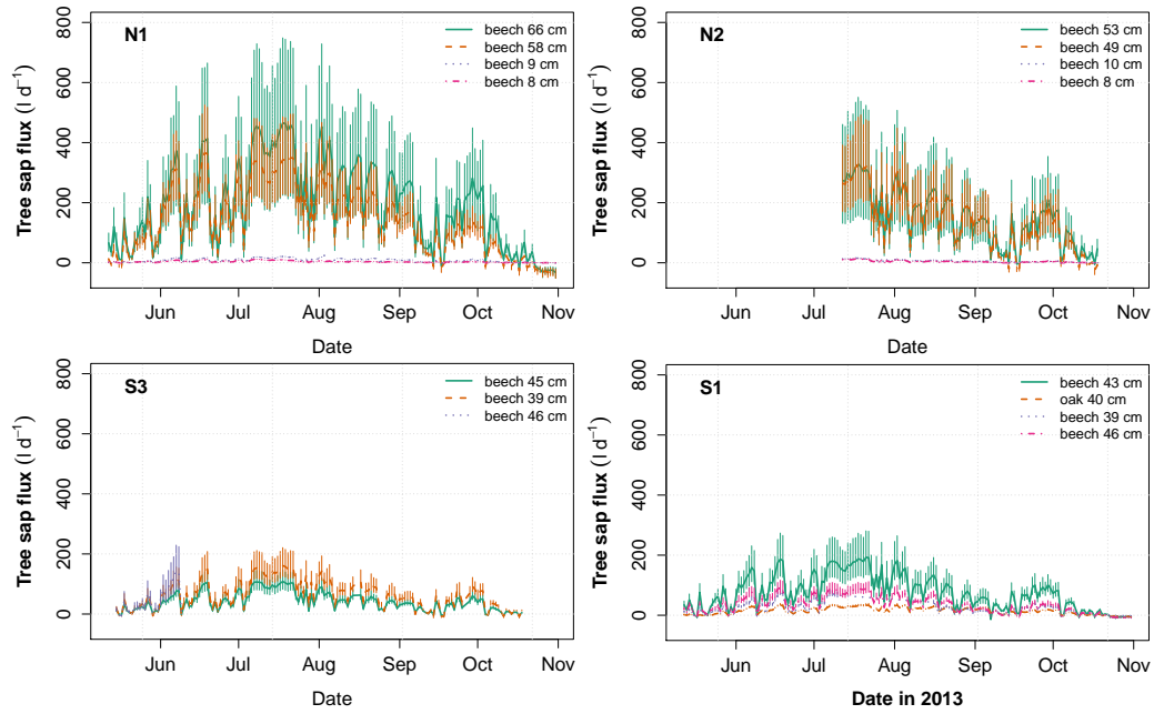
Figure S7: Daily tree-based sap flux rates for each tree (color coded) for the growing season in 2013 at site N1, N2, S3 and S1. Sap flux was obtained by integrating the product of measured SFD and the representative area of each reading at a sensor depth. The bold lines represent a linear decline of SFD towards the estimated heartwood radius. The thin vertical lines represent the minimal and maximal sap flux density profiles in the inner sapwood, see main text section 2.6
