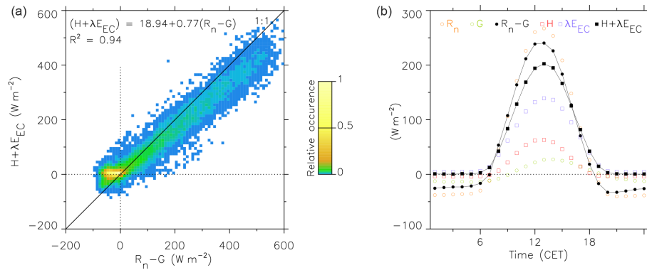
Figure 4. (a) Sum of turbulent fluxes (i.e., sum of sensible heat flux H and latent heat flux \lambda E_{EC} ; H + \lambda E_{EC} ) vs. the available energy (i.e., net radiation R_n minus surface soil heat flux G ; R_n - G ) and (b) mean daily pattern of the energy balance components. Graphs are based on measured hourly values (i.e., excluding gap-filled data, and masked for precipitation and wind directions affected by the tower) for the time period 1 June 2009–31 December 2015.
