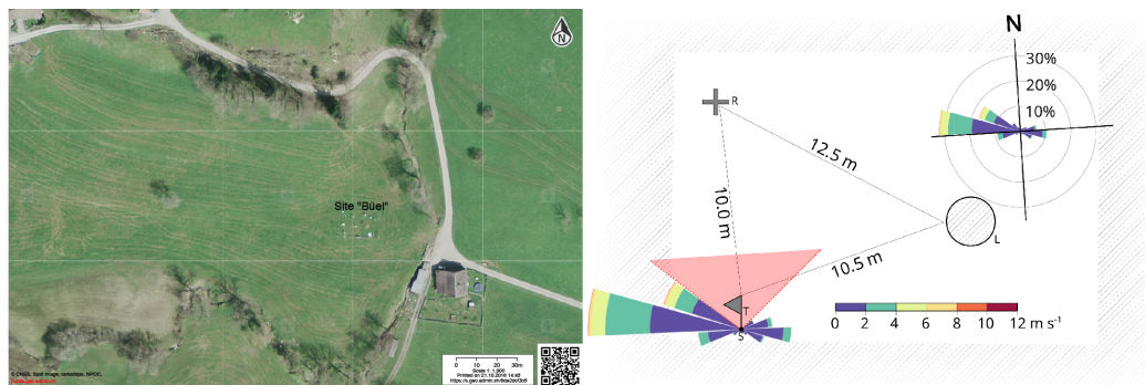
Figure 2. Left panel: aerial map of the site (see https://s.geo.admin.ch/6de2dcf3b5 for an interactive online version of the map) and right panel: schematics of the EC tower (denoted T), lysimeter (L), and radiation (R) measurement setup as well as the frequency of wind direction and velocity at the site “Büel” (white rectangle defines the area of the measurement field). The distance between the tower and the sonic (S) volume equals 1.17 m. The wind sector obstructed by the tower and the IRGA is highlighted in red and masked for the analyses (from 310 to 50°). The identical hatching of the surrounding grassland and the lysimeter surface indicates that the latter is treated according to the former (see text for details).
