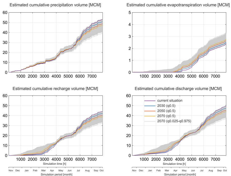
Figure 7. Impacts of the median climate scenarios ( q0.5 ) for years 2030, 2050 and 2070 as well as the uncertain climate scenarios (1000 random sampled combinations) for 2070 on the simulated precipitation, evapotranspiration, recharge and discharge for the studied catchment.
