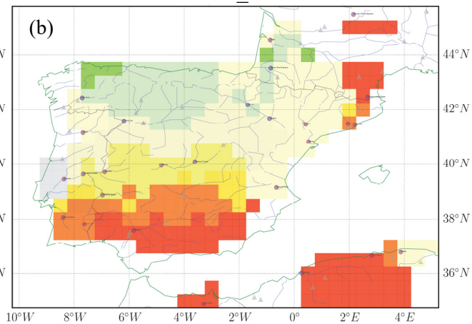
Norm_BIAS
