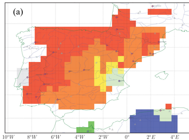
Correlation coefficient
