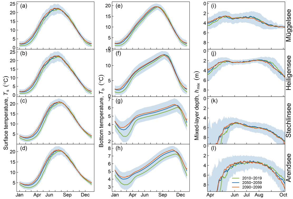
Figure 8. Modelled seasonal cycle of surface (a–d) and bottom temperature (e–h) and mixed-layer depth (i–l) in Müggelsee (a, e, i), Heiligensee (b, f, j), Stechlinsee (c, g, k), and Arendsee (d, h, l). Lines indicate decadal means and shading denotes 1 standard deviation each side of the mean.
