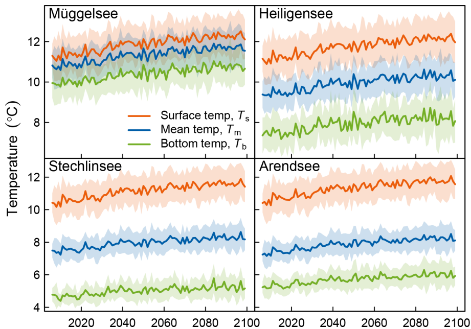
Figure 7. Projected evolution of surface, mean, and bottom temperatures in the four study lakes. Shading indicates 1 standard deviation either side of the mean.
