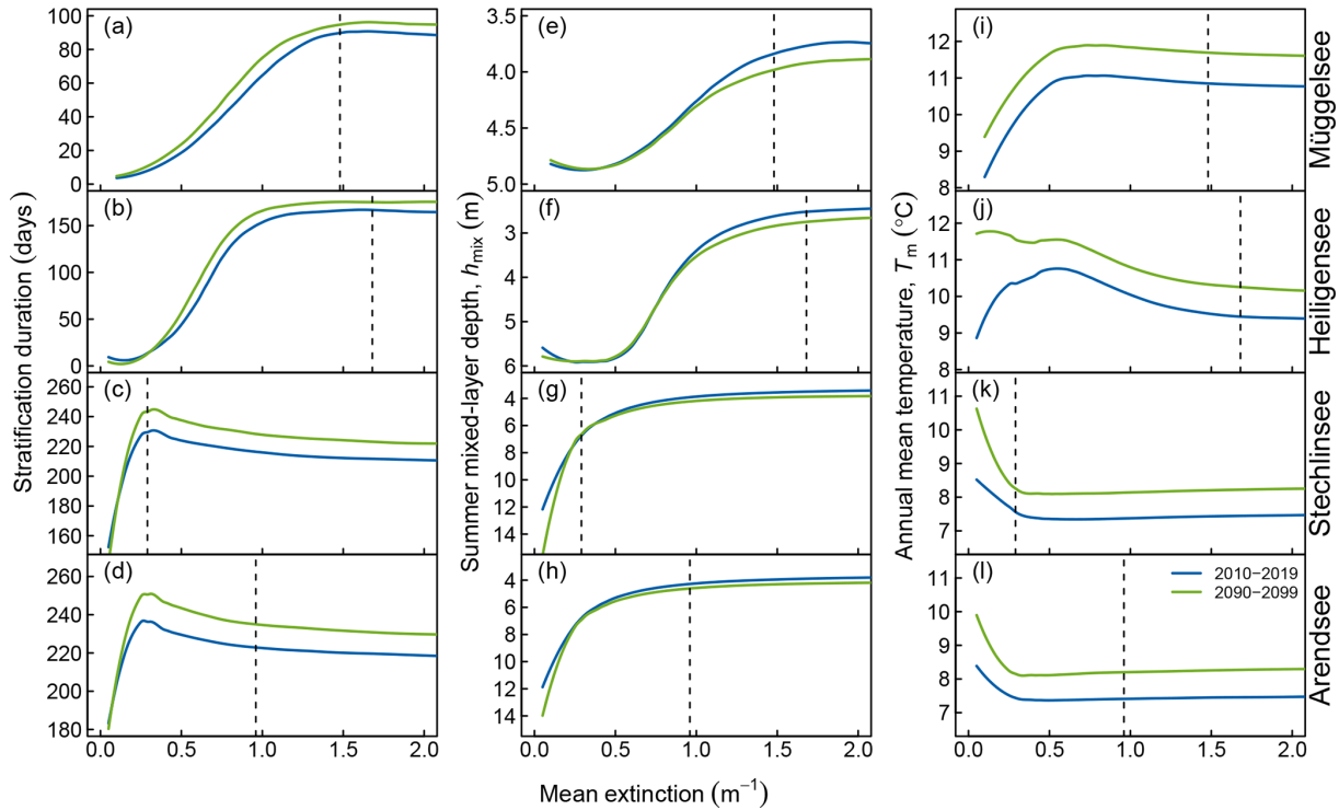
Figure 10. Interacting effects of extinction and warming on stratification duration (a–d), mean mixed-layer depth in summer (e–h), and annual mean temperature (i–l) in Müggelsee (a, e, i), Heiligensee (b, f, j), Stechlinsee (c, g, k), and Arendsee (d, h, l). Lines have been loess-smoothed and show ensemble means for the decades 2010–2019 (blue) and 2090–2099 (green) as a function of extinction. Black vertical dashed lines show the long-term measured extinction in each lake.
