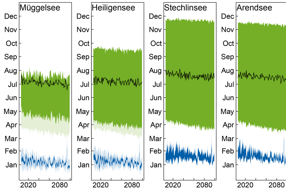
Figure 9. Projected trends in stratification in the four study lakes. Green shading shows summer stratification, blue shows winter stratification. Lighter shading indicates intermittent stratification. The black line shows the timing of maximum surface temperature. The model was forced with the baseline (historical) transparency.
