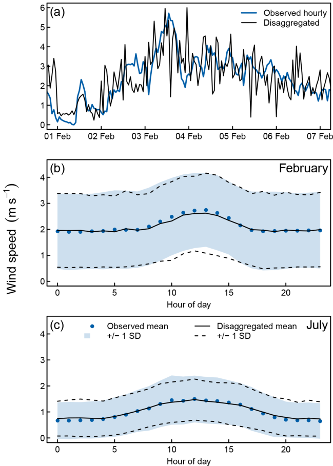
Figure 3. Comparison of disaggregated and observed sub-daily wind speeds at the Menz weather station (5 km from Stechlinsee): sample of observed hourly wind data from 1998 and the disaggregated wind speeds generated from the corresponding daily means (a); hourly mean and standard deviation of observed (circles, shaded area) and disaggregated wind speeds (solid and dashed lines) in February (b) and July (c).
