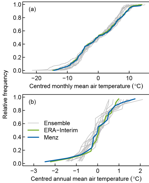
Figure 2. Cumulative distribution function of centred monthly (a) and annual mean air temperature (b), based on data from 1991 to 2010. The grey lines show the 12 historical scenarios in the ensemble, the green line shows ERA-Interim reanalysis data, and the blue line shows the observed data from the Menz weather station. All data are for the closest pixel or weather station to Stechlinsee.
