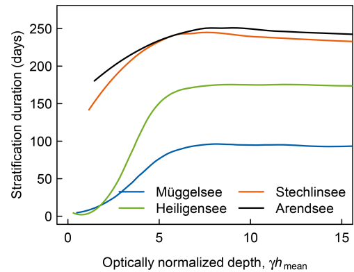
Figure 11. Stratification duration vs. optically normalized depth (mean extinction ( \gamma , \text{m}^{-1} ) \times mean depth ( h_{\text{mean}} , m), dimensionless) in lakes Müggelsee, Heiligensee, Stechlinsee, and Arendsee. The curves are loess-smoothed and are based on ensemble simulations with the baseline extinction in each lake for the 2090–2099 period.
