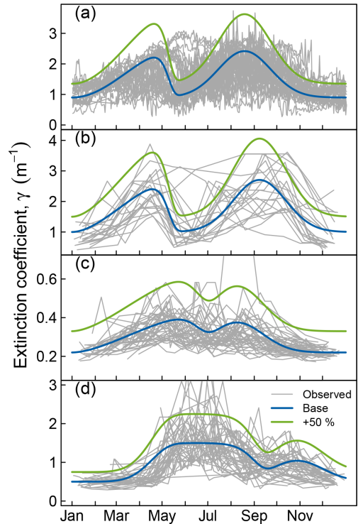
Figure 4. Seasonal course of extinction ( \gamma ) in Müggelsee (a), Heiligensee (b), Stechlinsee (c), and Arendsee (d). Grey lines show superimposed observed extinction during individual years, thick blue lines show the idealized seasonal course of extinction used in model simulations with FLake (base scenario). Green lines show base extinction increased by 50%. Panels (a) and (b) modified from Shatwell et al. (2016).
