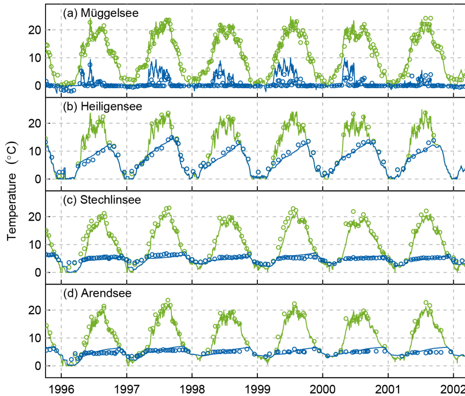
Figure 5. Comparison of modelled (lines) and observed temperatures (points) in Müggelsee (a), Heiligensee (b), Stechlinsee (c), and Arendsee (d). Green lines and symbols show surface temperatures, blue lines and symbols show bottom temperatures (b–d) or surface–bottom temperature differences (a).
