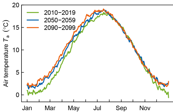
Figure 6. Projected changes in over-lake near-surface air temperature under RCP4.5. Lines show decadal means over all climate projections and all four locations.
