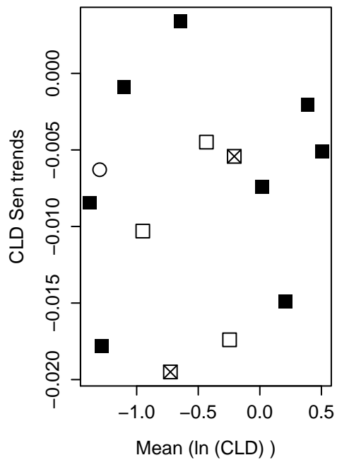
(a) Soil
