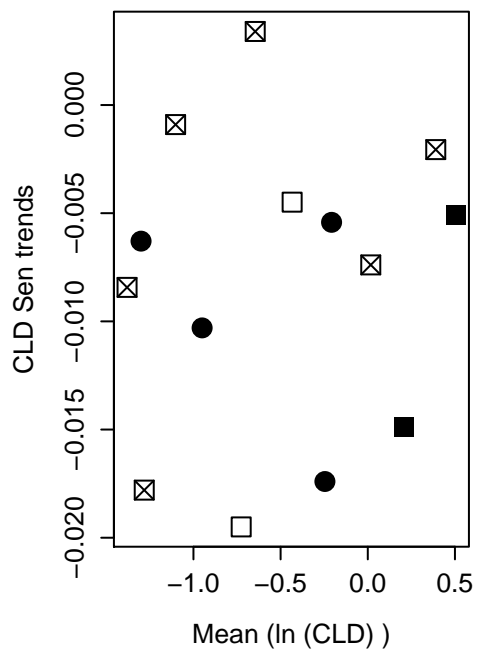
(b) Geology
