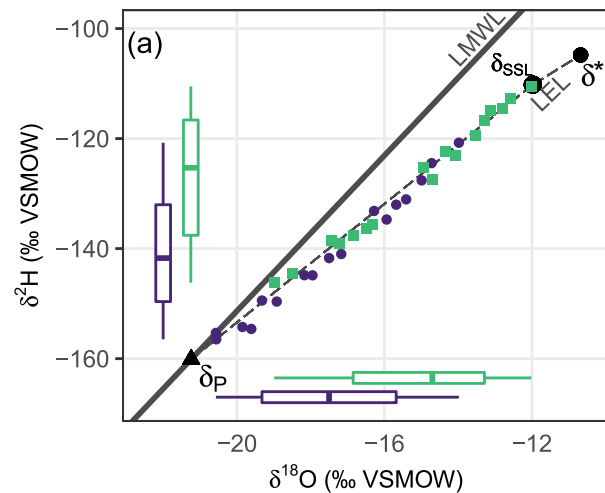
Correction of Pre-Snowmelt Samples for Ice-Fractionation
