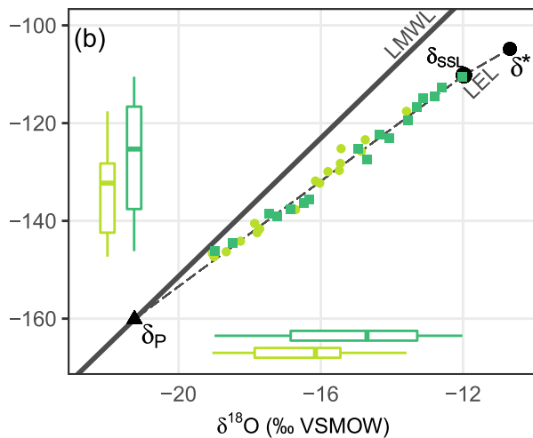
Pre-Snowmelt and Post-Snowmelt Lake Samples
