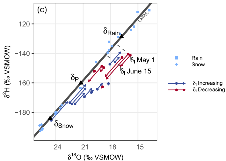
Change in \delta_i from Pre-Snowmelt to Post-Snowmelt
