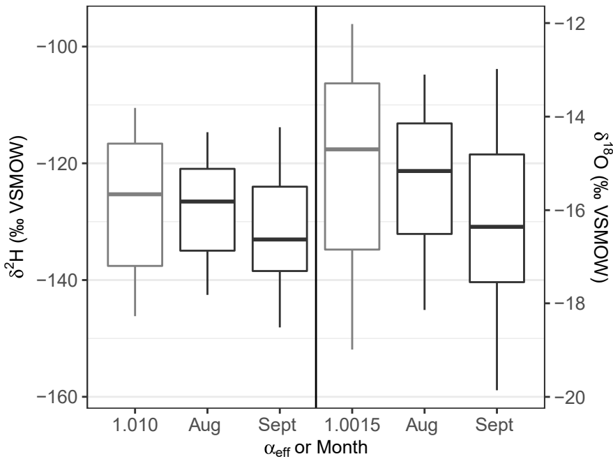
Comparison of Corrected Pre-Ice and Fall 2018 Lake Isotope Values
