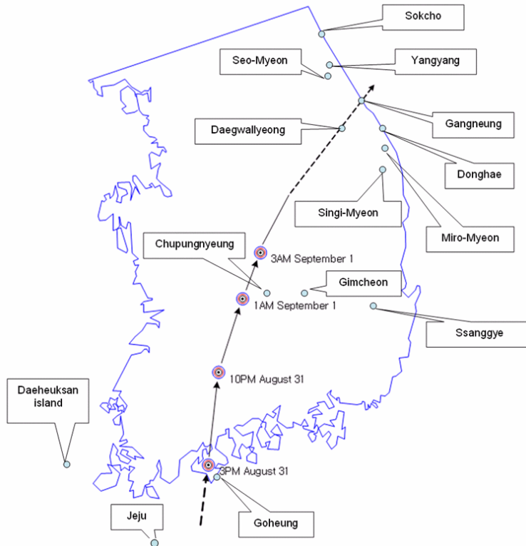
Fig. 2. Path of typhoon in South Korea.
