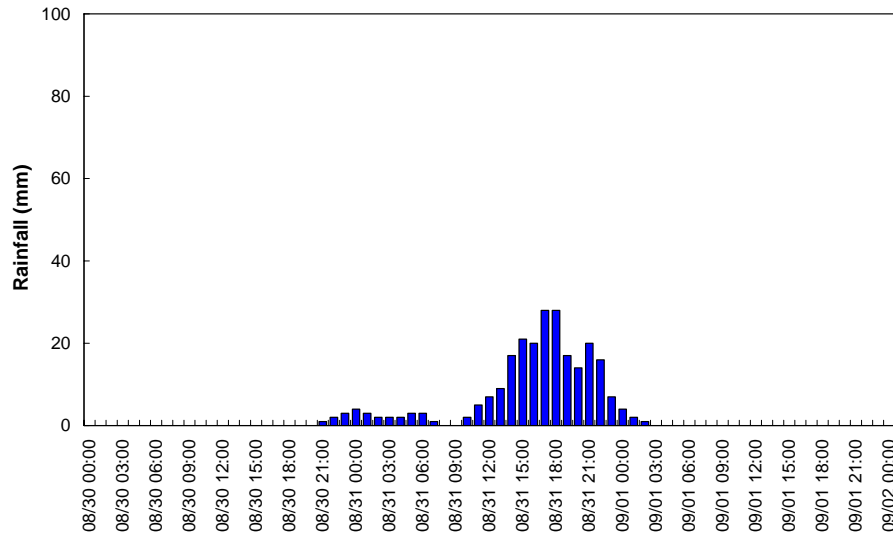
Fig. 5. Time distribution of rainfall in Gimcheon area (b) Gimcheon.
