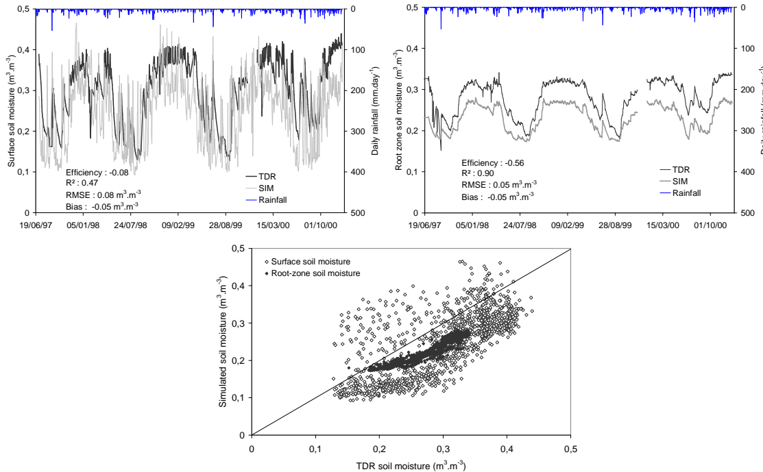
Fig. 3. Surface soil moisture (top left) and root-zone soil moisture (top right) and drawn together (bottom) measured by TDR and simulated by SIM model from June 1997 to November 2000.
