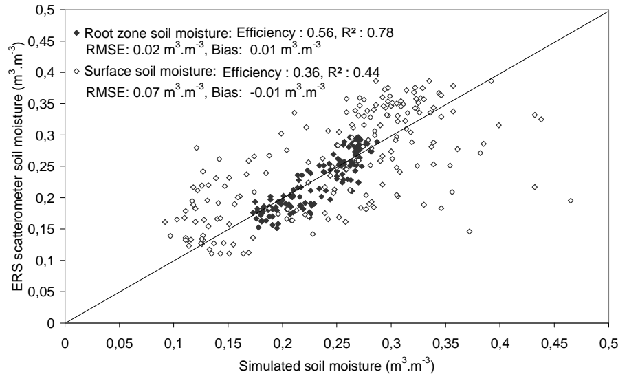
Fig. 4. Comparison of surface and root-zone soil moisture ( \text{m}^3 \text{m}^{-3} ) for ERS scatterometer data (5 cm and 1 m depth, respectively) and simulation (1 cm and 1.5 m depth, respectively), from June 1997 to November 2000.
