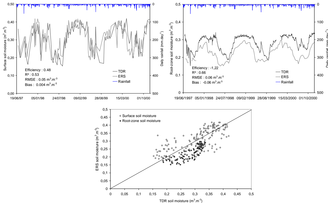
Fig. 2. Surface soil moisture (top left) and root-zone soil moisture (top right) and drawn together (bottom) measured by TDR and obtained by ERS scatterometer from June 1997 to November 2000.
