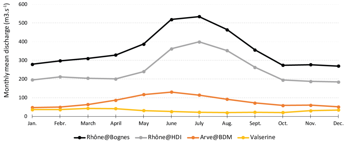
Fig. 1. hydrograms of the Rhône@Bognes, Rhône@HDI, Arve@BDM and for Valserine catchment for the 1923-2010 period.
