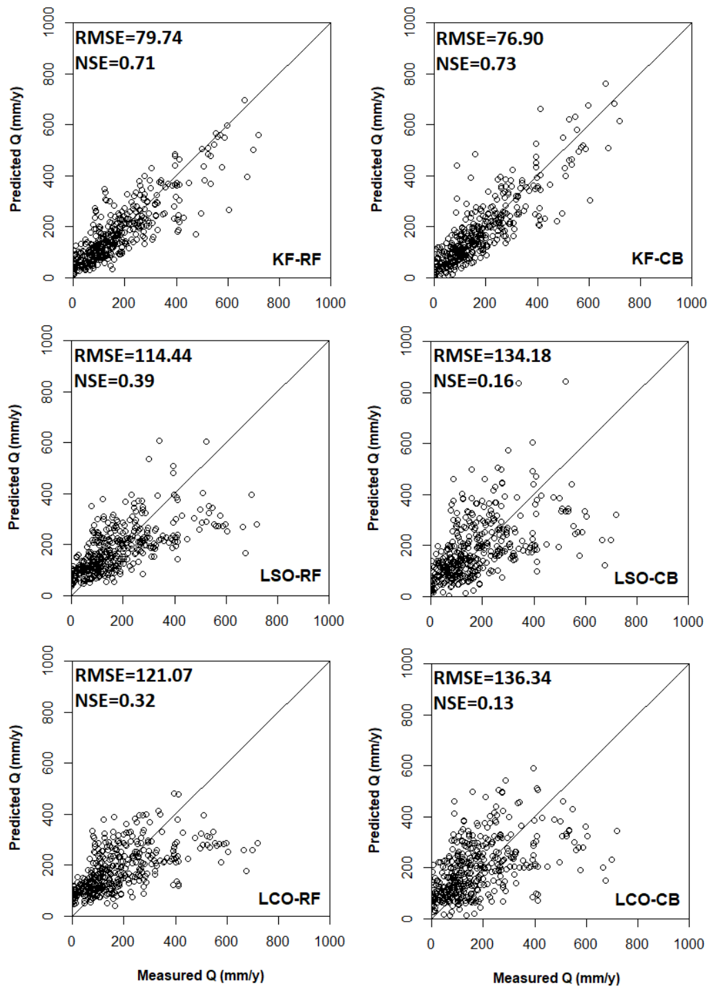
Figure 3. Model performance of KF-RF: K-Fold cross-validated random forest model, KF-CB: k-fold cross-validated Cubist model, LSO-RF: Leave station out cross-validated random forest model, LSO-CB: Leave station out cross-validated cubist model, LCO-RF: Leave cluster out cross-validated random forest model, LCO-CB: Leave cluster out cross-validated cubist model, when models was ran after excluding DEM.
