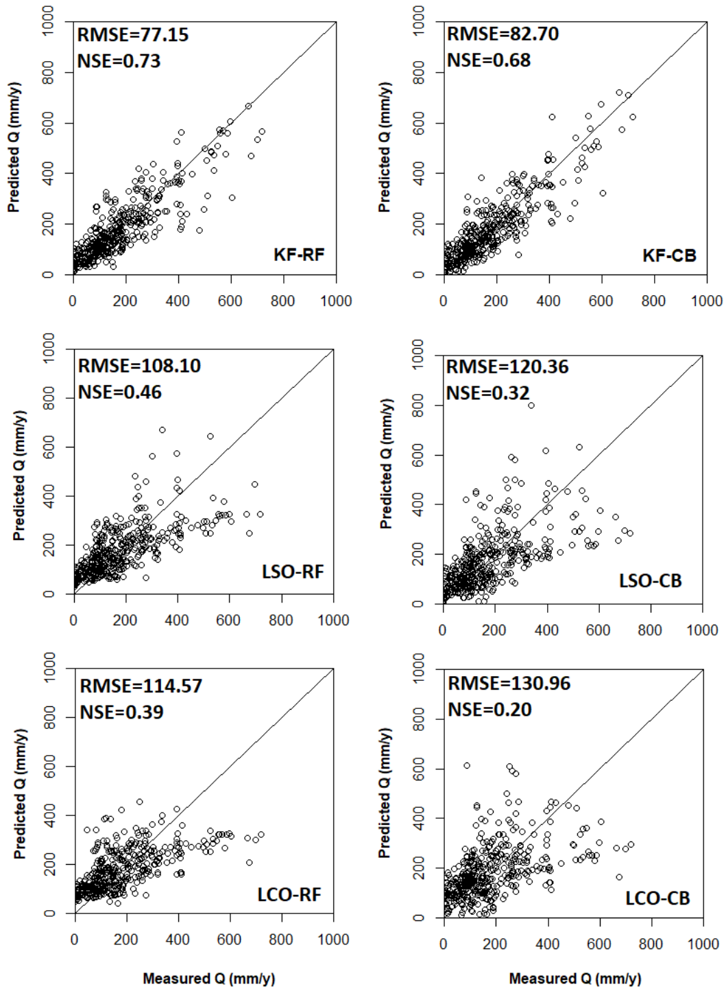
Figure 1. Model performance of KF-RF: K-Fold cross-validated random forest model, KF-CB: k-fold cross-validated Cubist model, LSO-RF: Leave station out cross-validated random forest model, LSO-CB: Leave station out cross-validated cubist model, LCO-RF: Leave cluster out cross-validated random forest model, LCO-CB: Leave cluster out cross-validated cubist model, when models was ran with precipitation (P) instead of Db.
