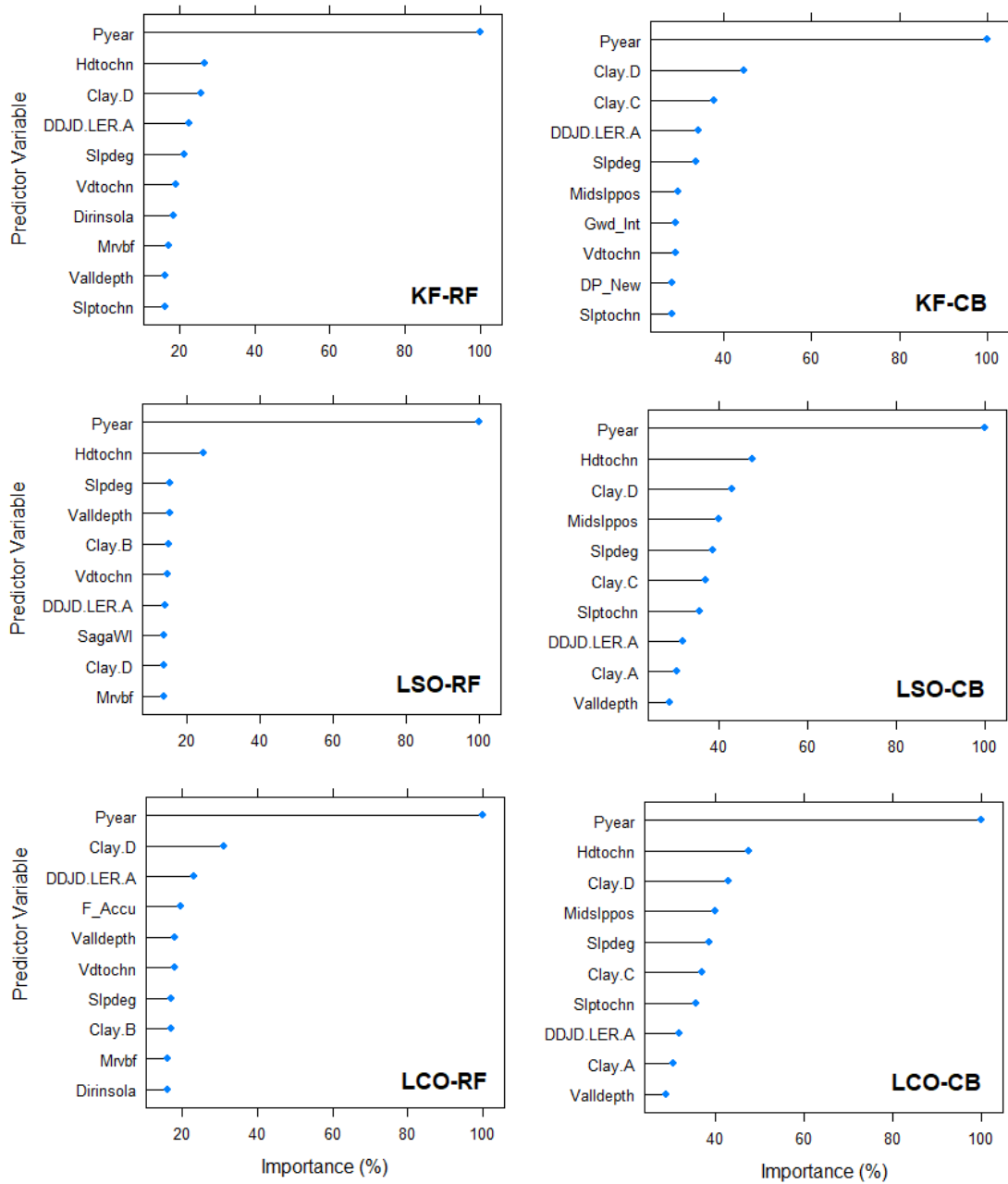
Figure 4. Top 10 most important covariates for KF-RF: K-Fold cross-validated random forest model, KF-CB: k-fold cross-validated Cubist model, LSO-RF: Leave station out cross-validated random forest model, LSO-CB: Leave station out cross-validated cubist model, LCO-RF: Leave cluster out cross-validated random forest model, LCO-CB: Leave cluster out cross-validated cubist model, when model was ran after excluding DEM.
