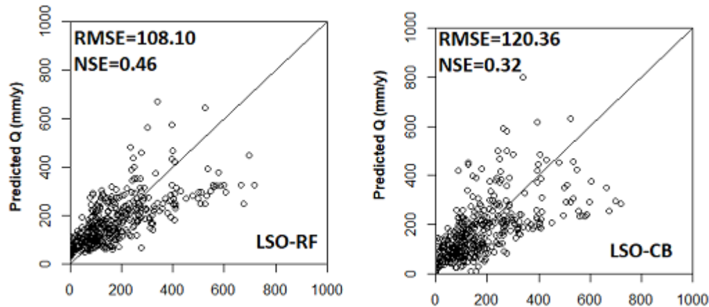
Fig. 2. Model performance of LSO-RF: Leave station out cross-validated random forest model, LSO-CB: Leave station out cross-validated cubist model with precipitation (P) instead of percolation (Db).
