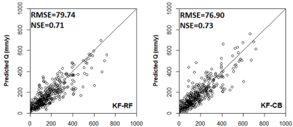
Fig. 7. Model performance of KF-RF: K-Fold cross-validated random forest model, KF-CB: k-fold cross-validated cubist model, when models was ran after excluding DEM.
