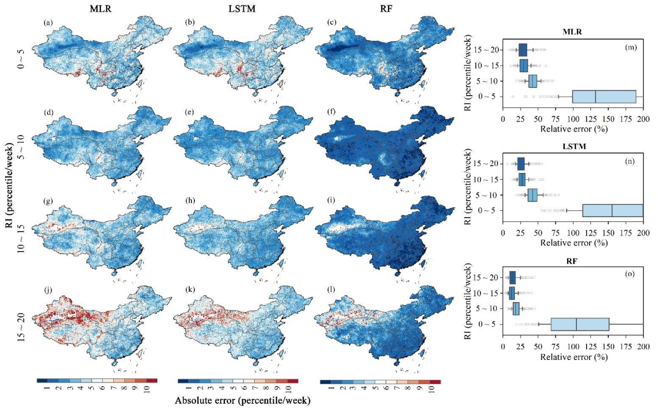
385 Figure 7: Spatial pattern of the absolute errors and boxplots of the relative errors of the RI estimated by the MLR, LSTM, and RF methods against observed RI at four percentile intervals.
