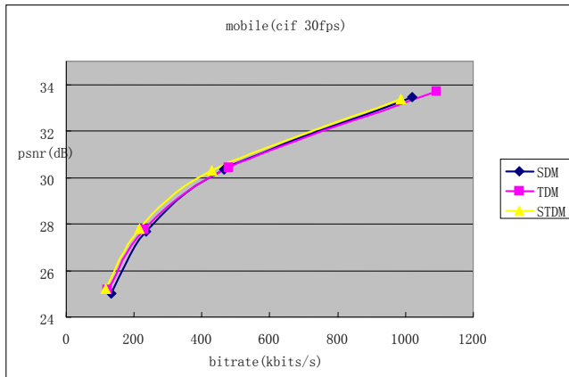
Figure 5. Rate-distortion curves for all pictures in Mobile sequence under regular B configuration
