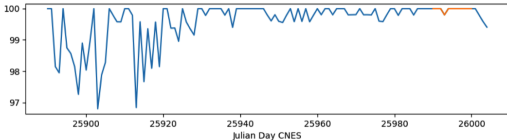
FIGURE : Fixing rates of GPS ambiguities for HY-2C.
