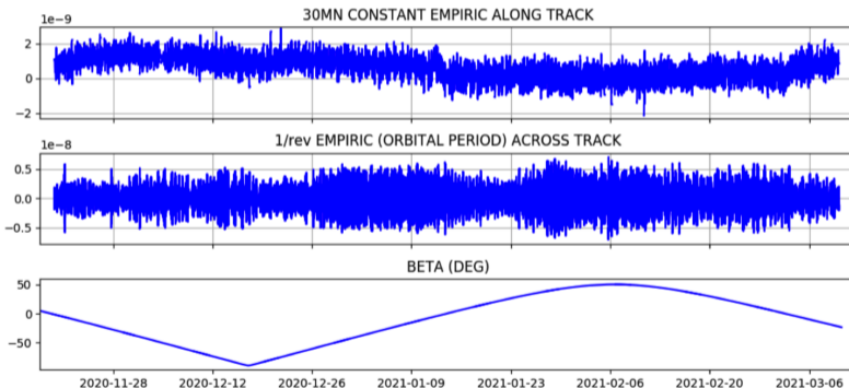
FIGURE : Empirical accelerations and beta angle for HY-2C.
