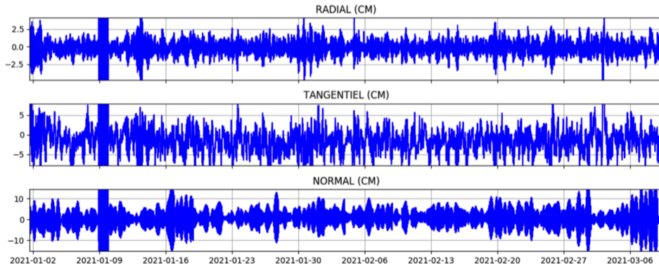
FIGURE : HY-2C MOE - POE orbits.
