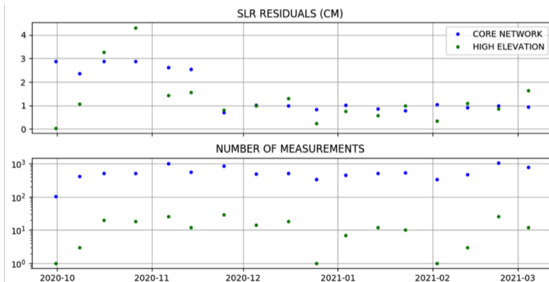
FIGURE : SLR residuals and tracking for HY-2C.
