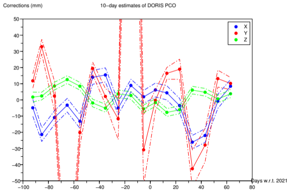
FIGURE : 10-day estimates of DORIS PCO.
