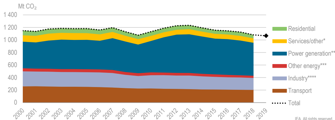
Figure 3.2 Japan’s energy-related CO 2 emissions by sector, 2000-19
